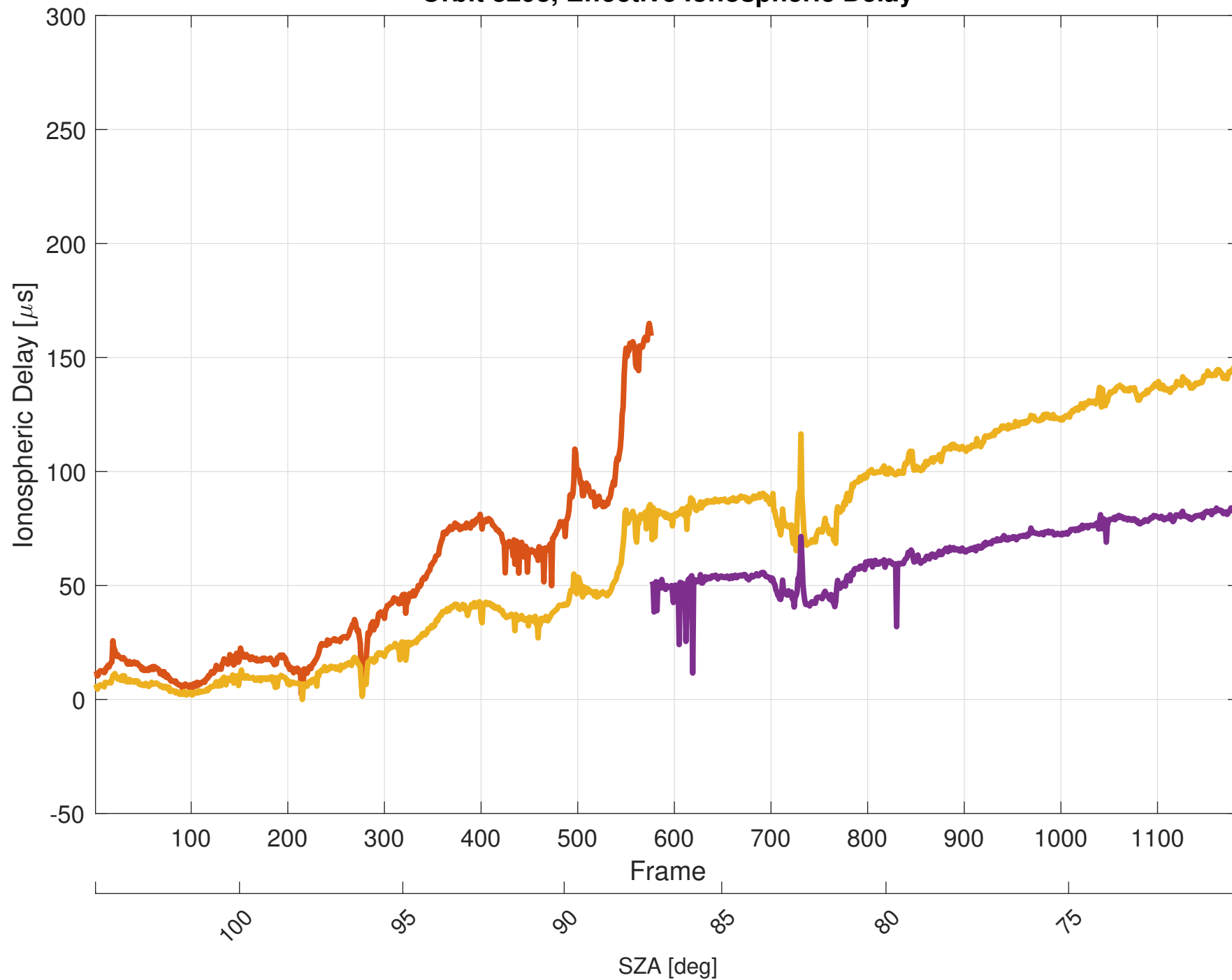
Orbit 8298, Effective Ionospheric Delay
