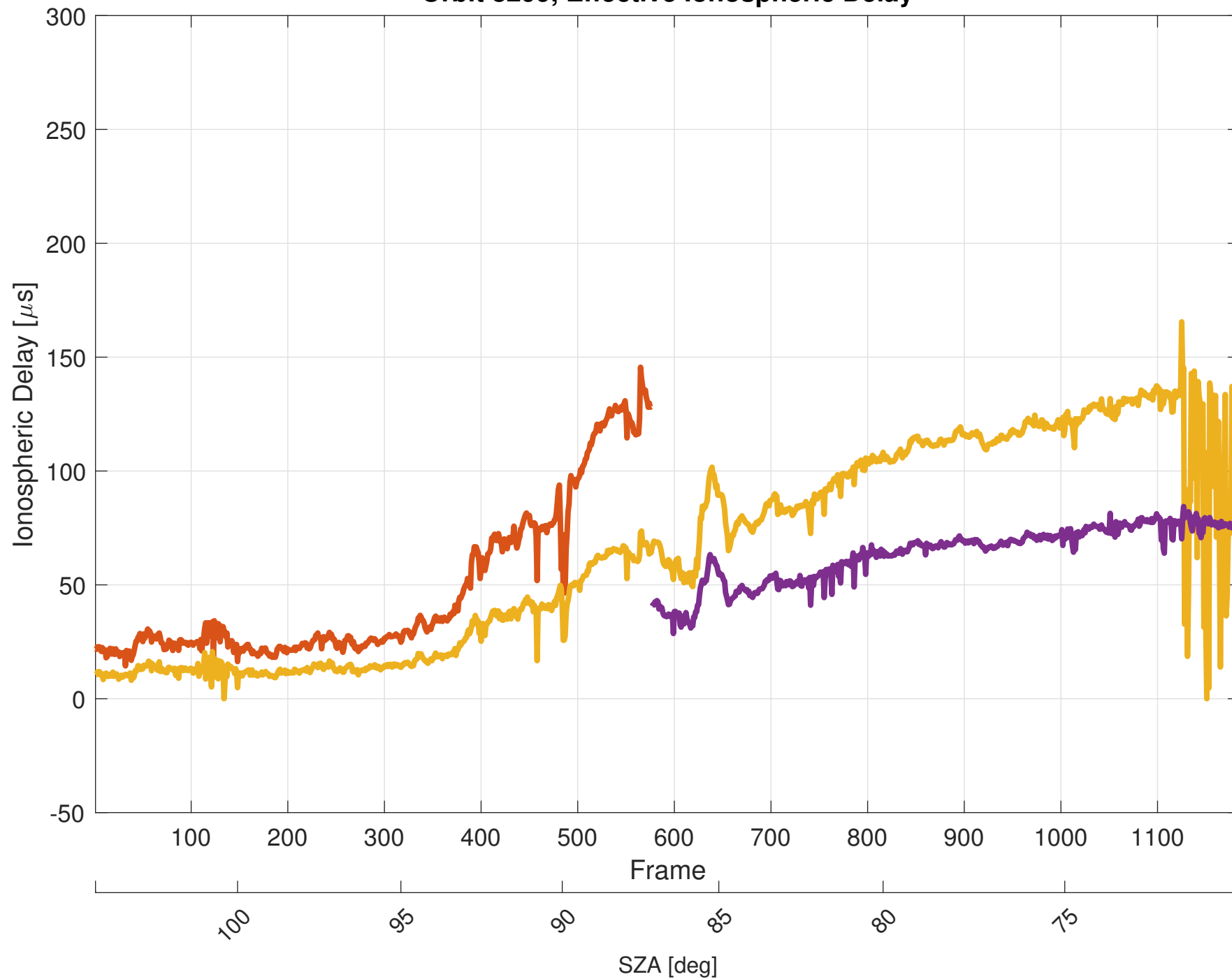
Orbit 8299, Effective Ionospheric Delay
