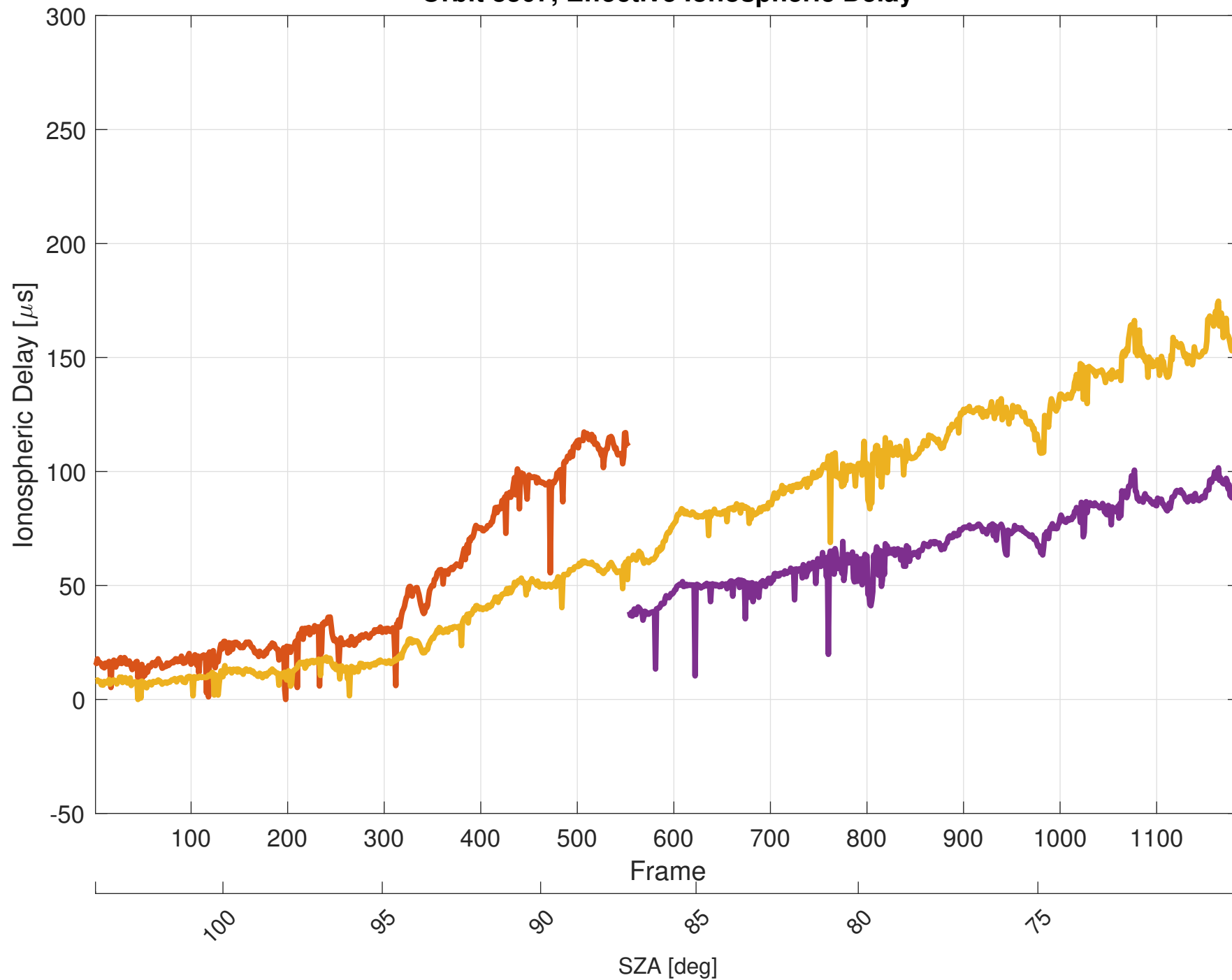
Orbit 8307, Effective Ionospheric Delay
