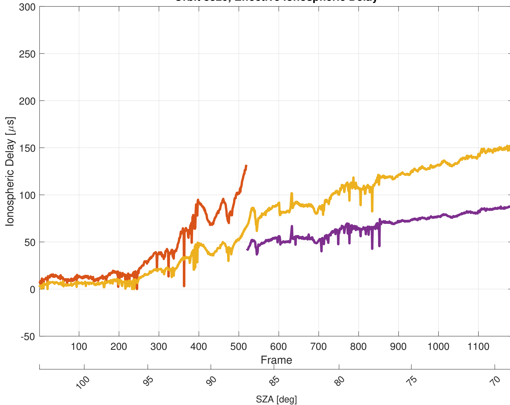
Orbit 8320, Effective Ionospheric Delay
