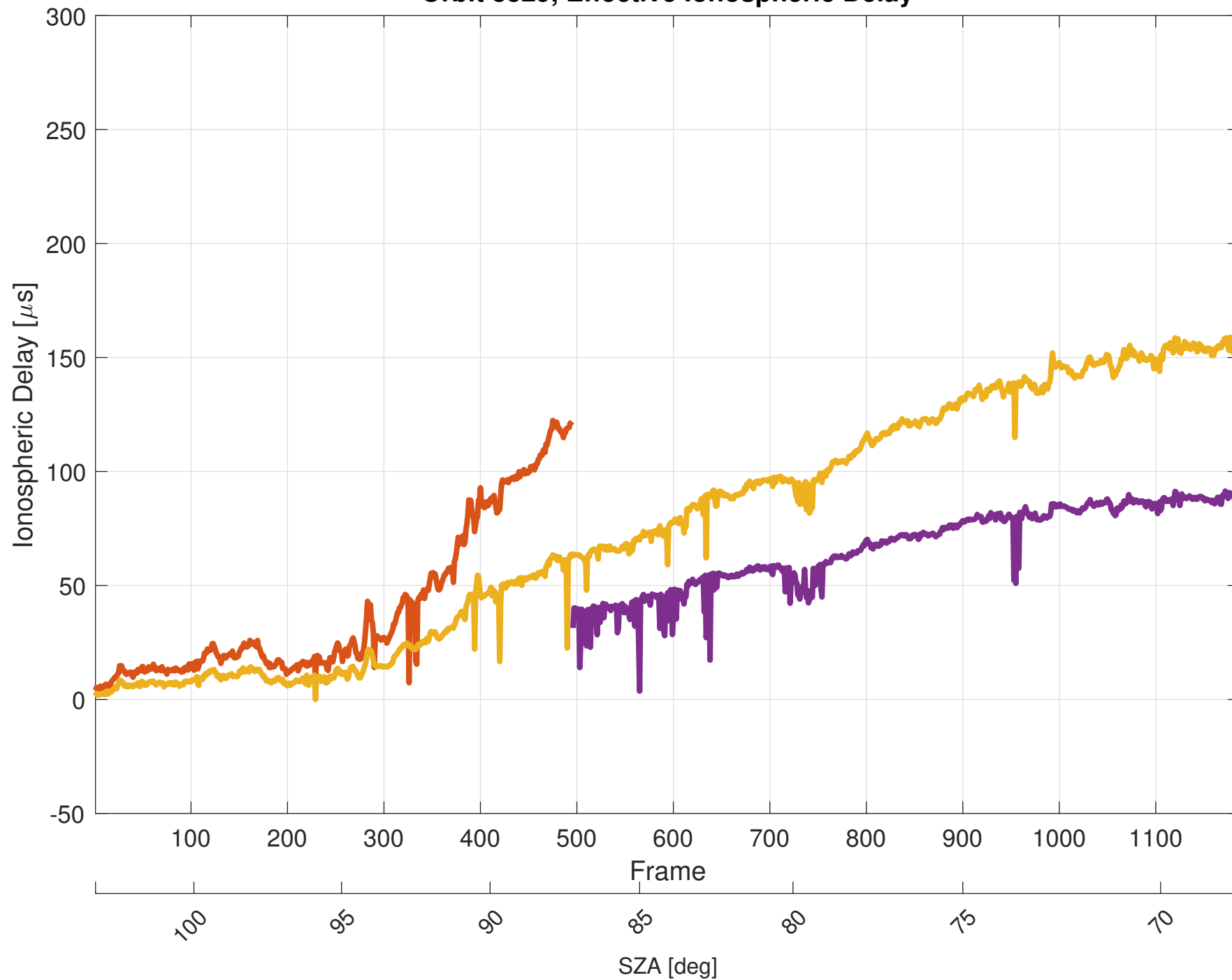
Orbit 8329, Effective Ionospheric Delay
