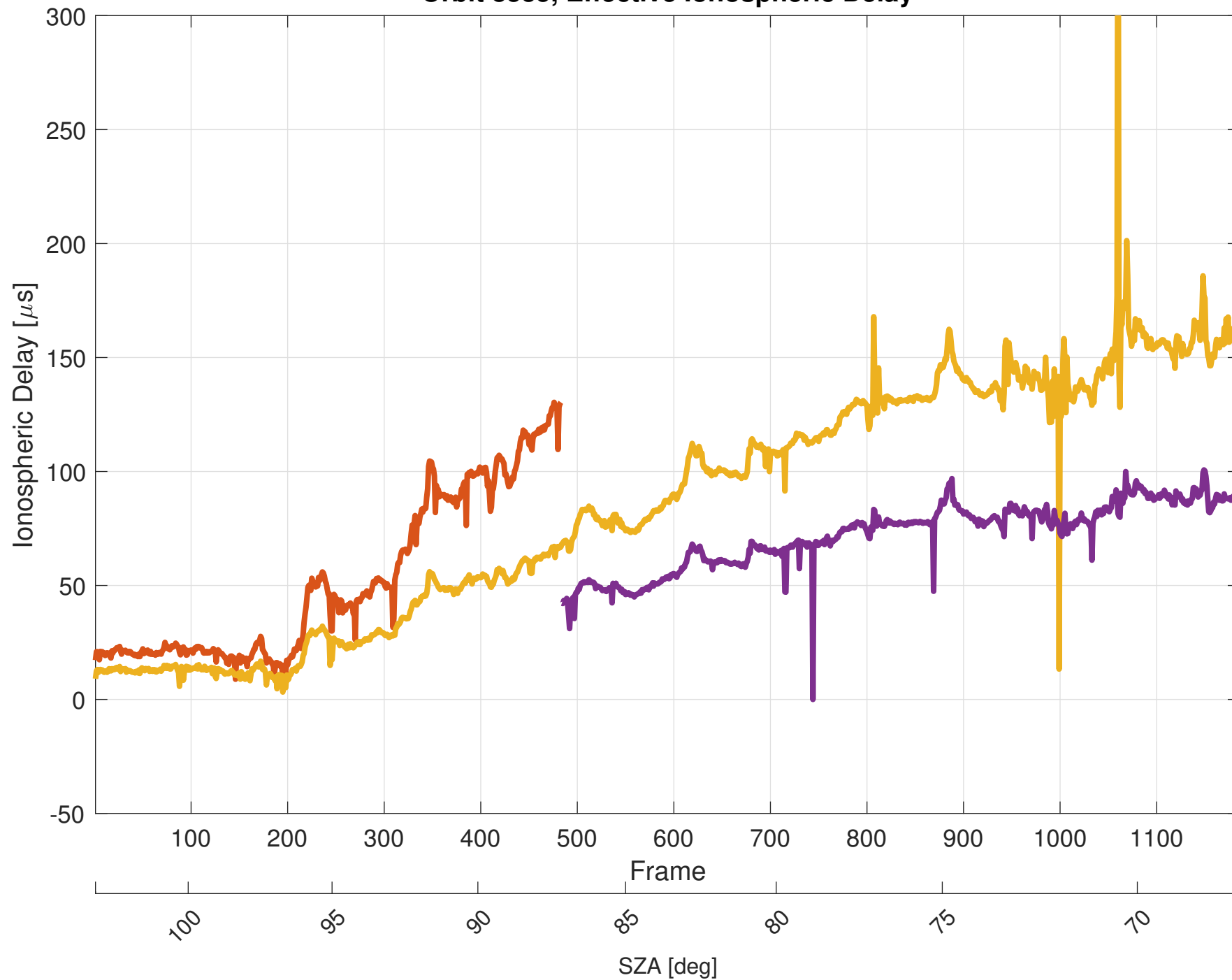
Orbit 8335, Effective Ionospheric Delay
