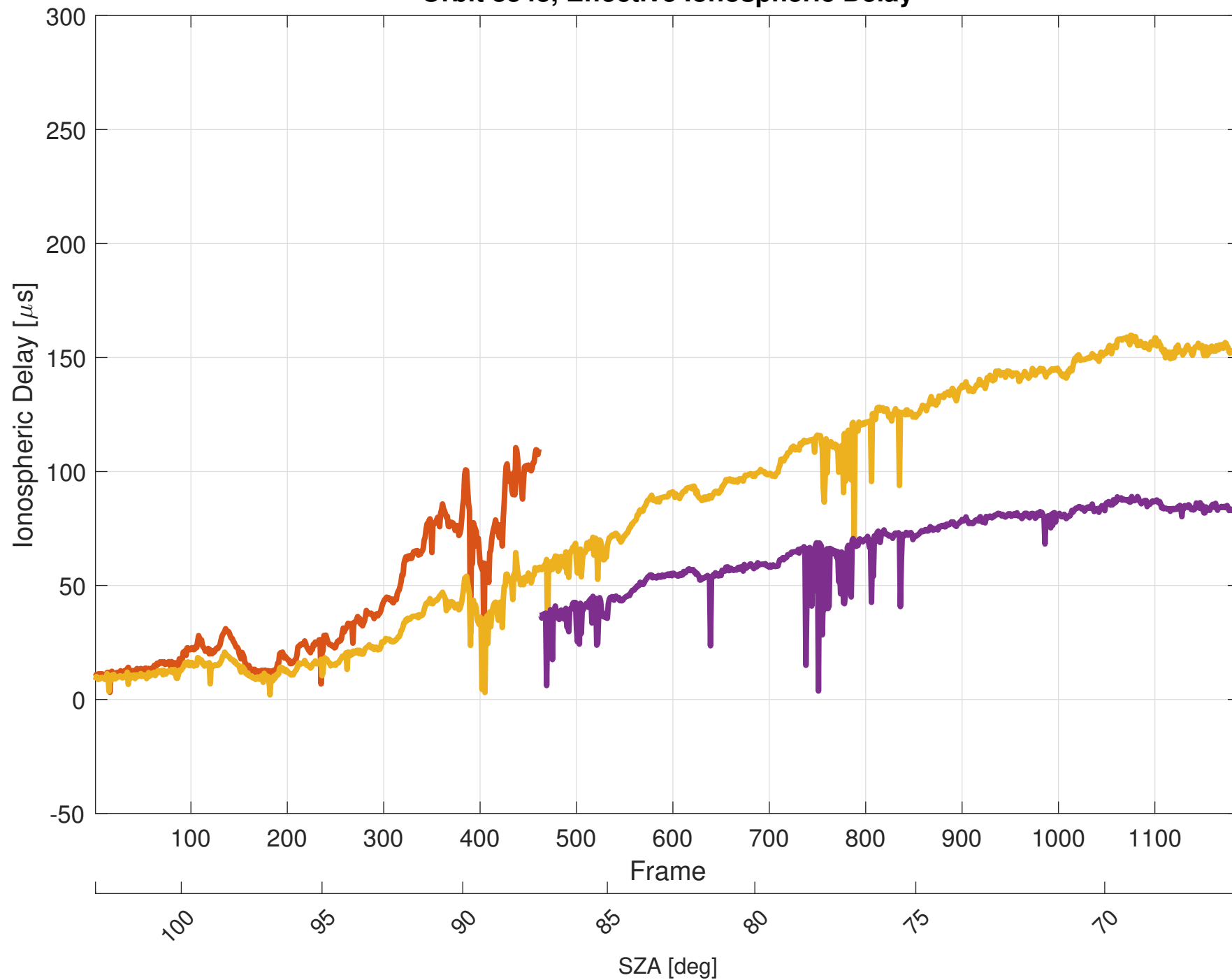
Orbit 8343, Effective Ionospheric Delay
