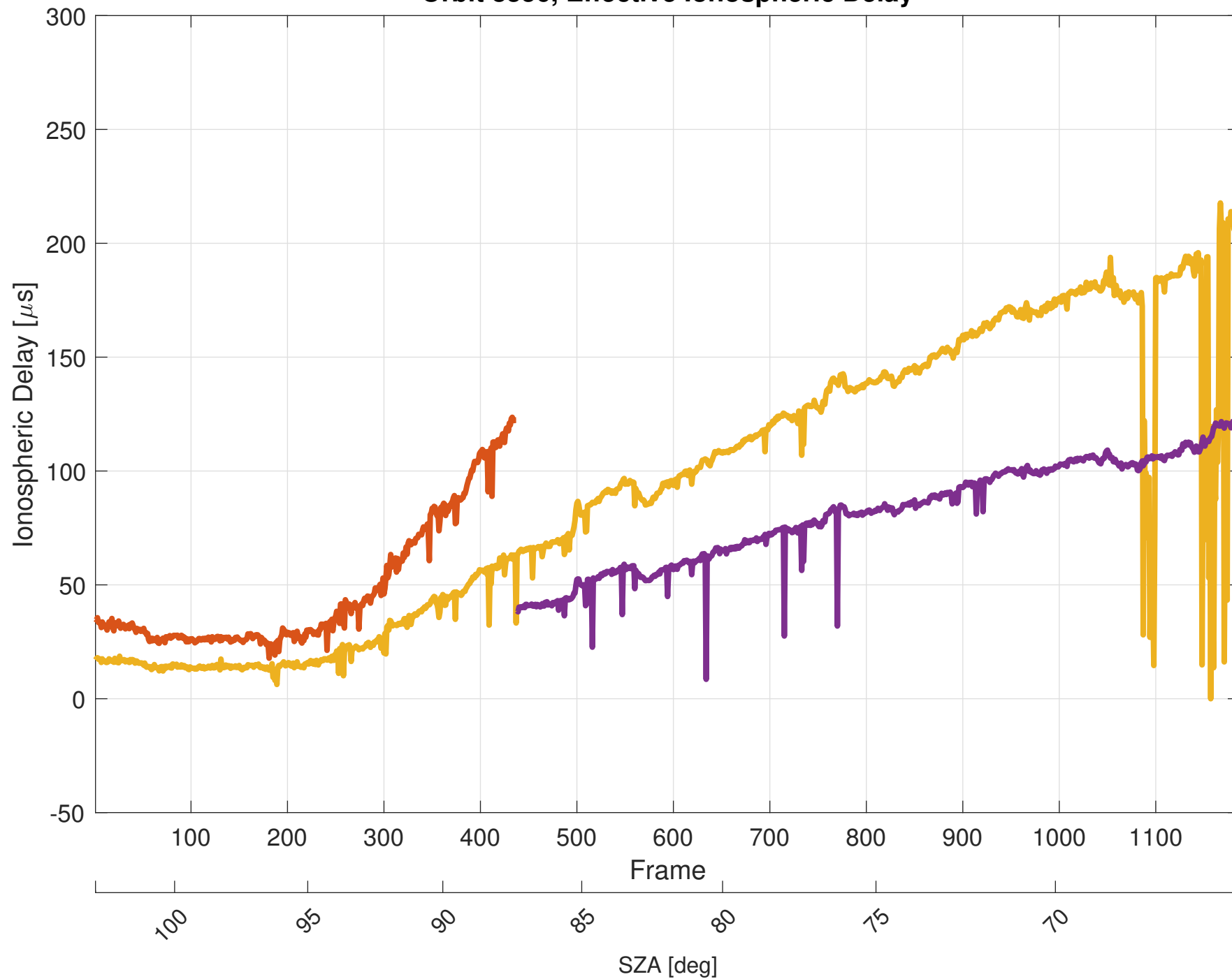
Orbit 8356, Effective Ionospheric Delay
