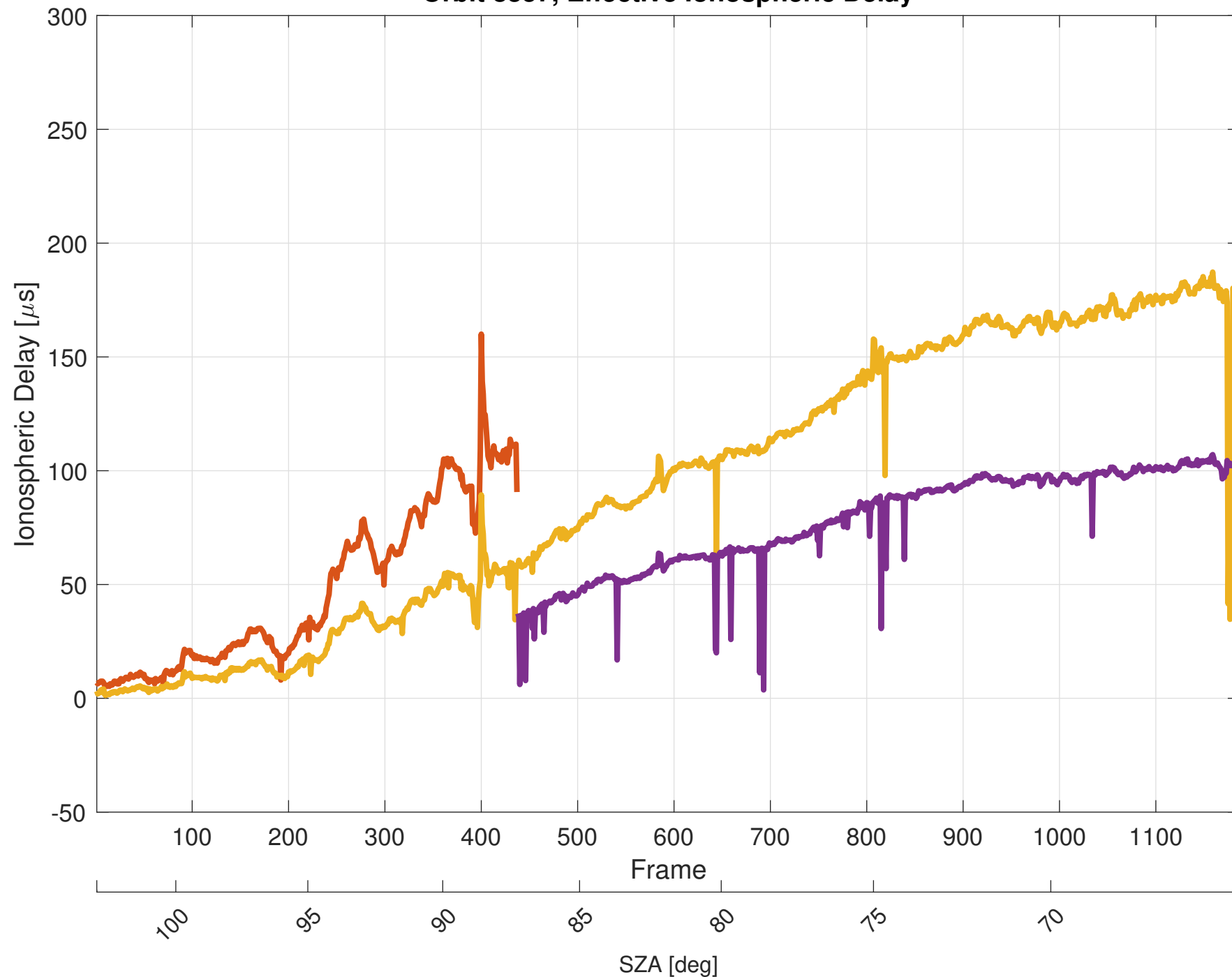
Orbit 8357, Effective Ionospheric Delay
