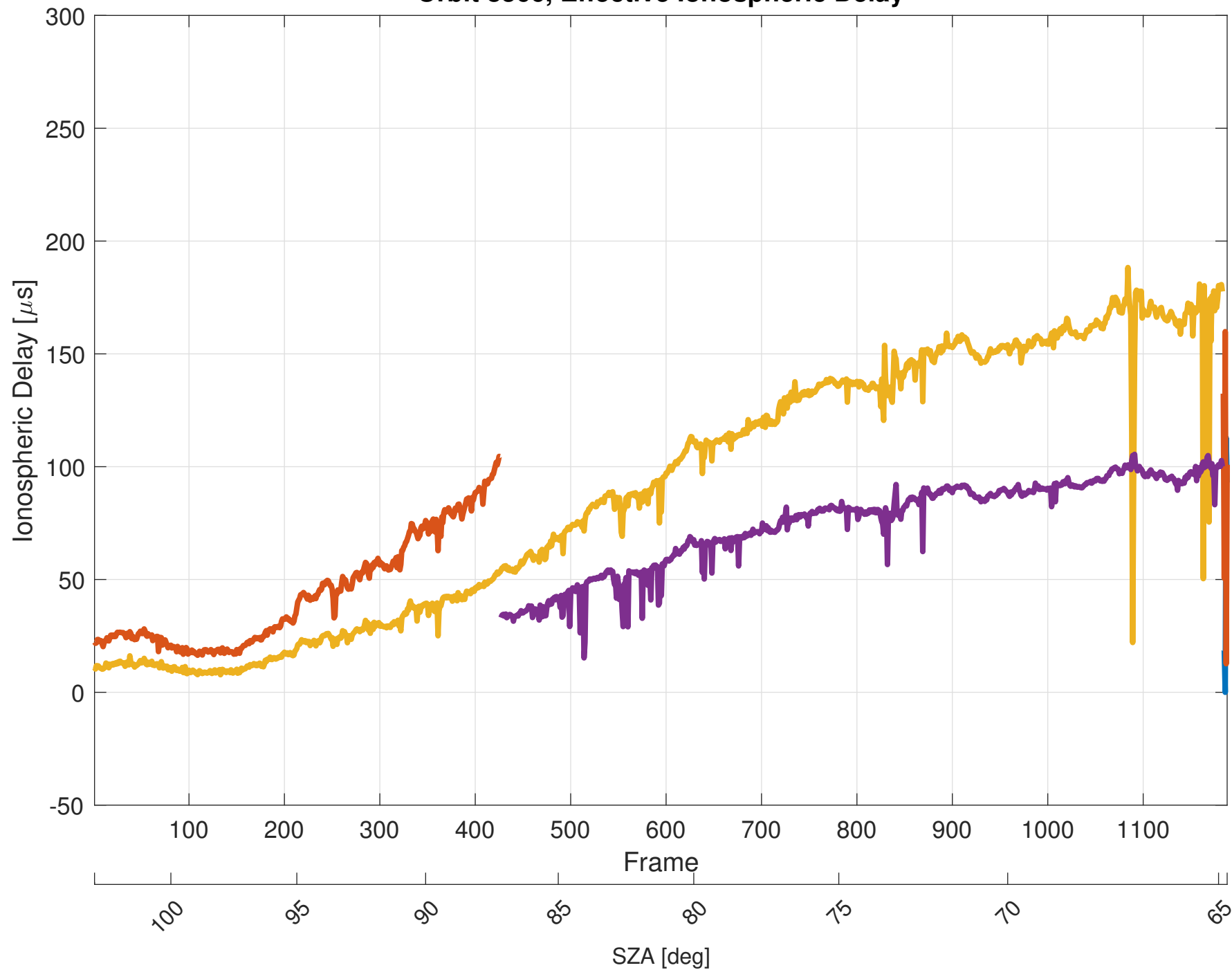
Orbit 8366, Effective Ionospheric Delay
