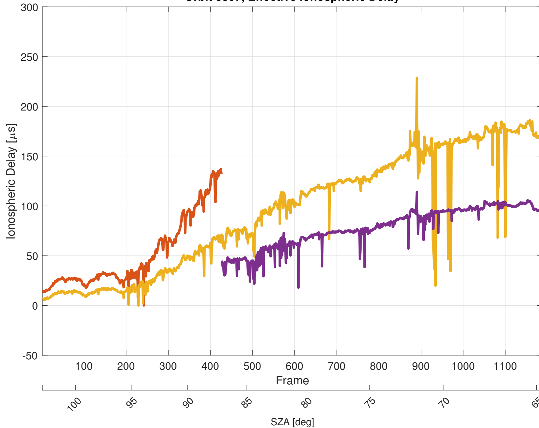
Orbit 8367, Effective Ionospheric Delay
