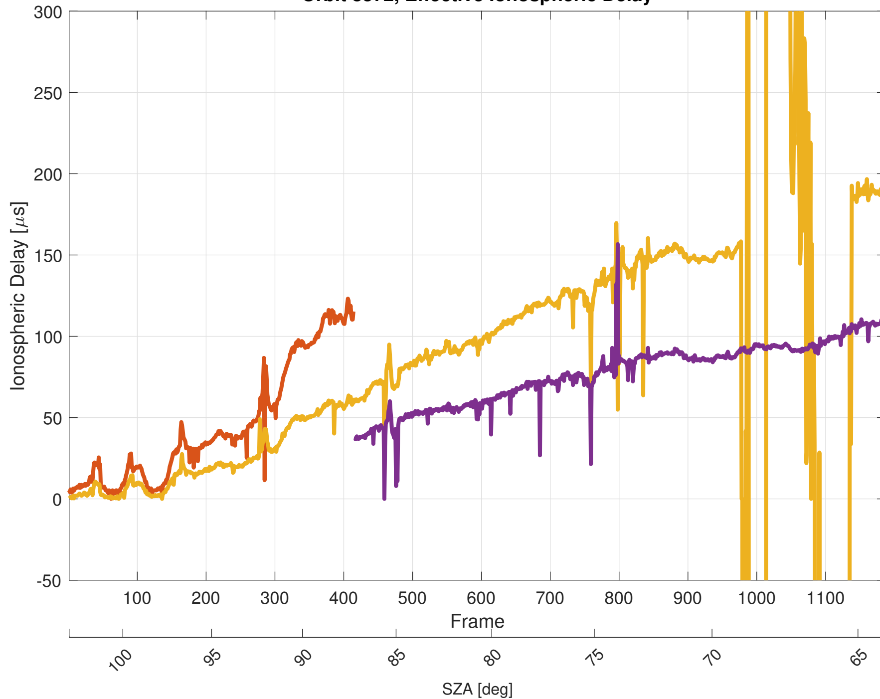
Orbit 8372, Effective Ionospheric Delay
