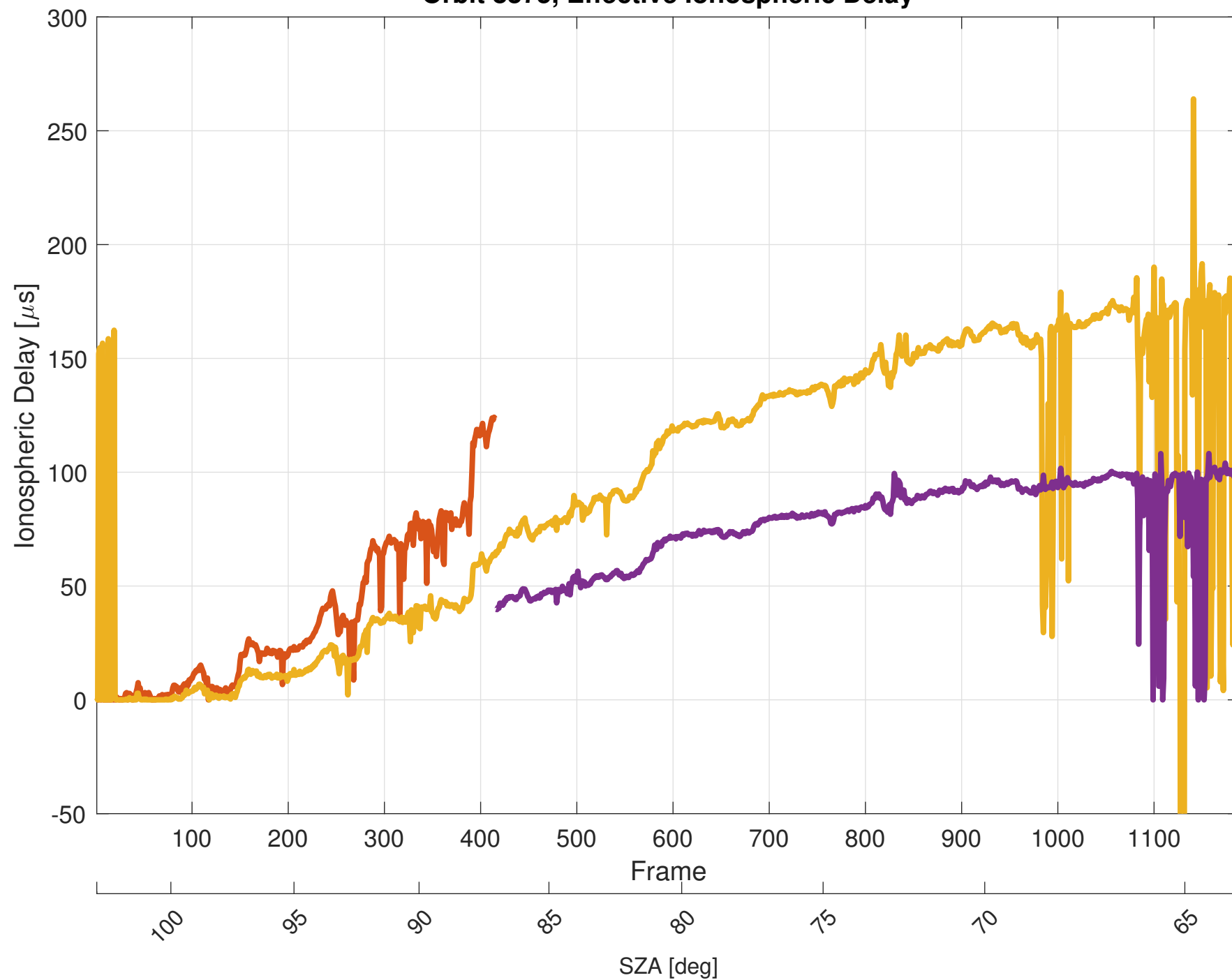
Orbit 8375, Effective Ionospheric Delay
