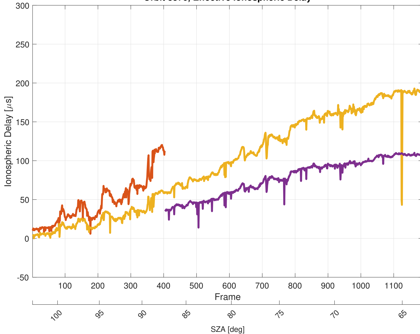
Orbit 8376, Effective Ionospheric Delay
