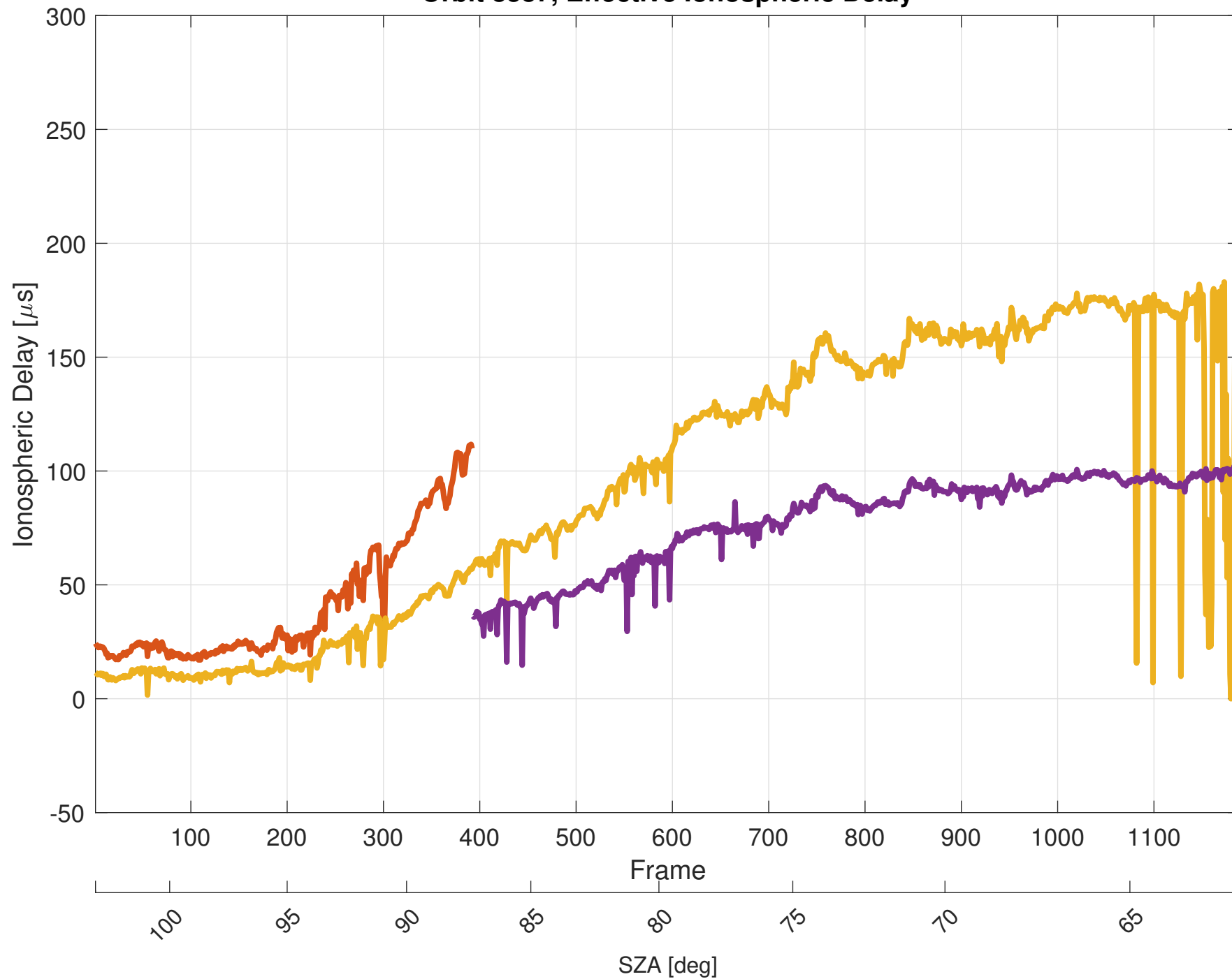
Orbit 8387, Effective Ionospheric Delay
