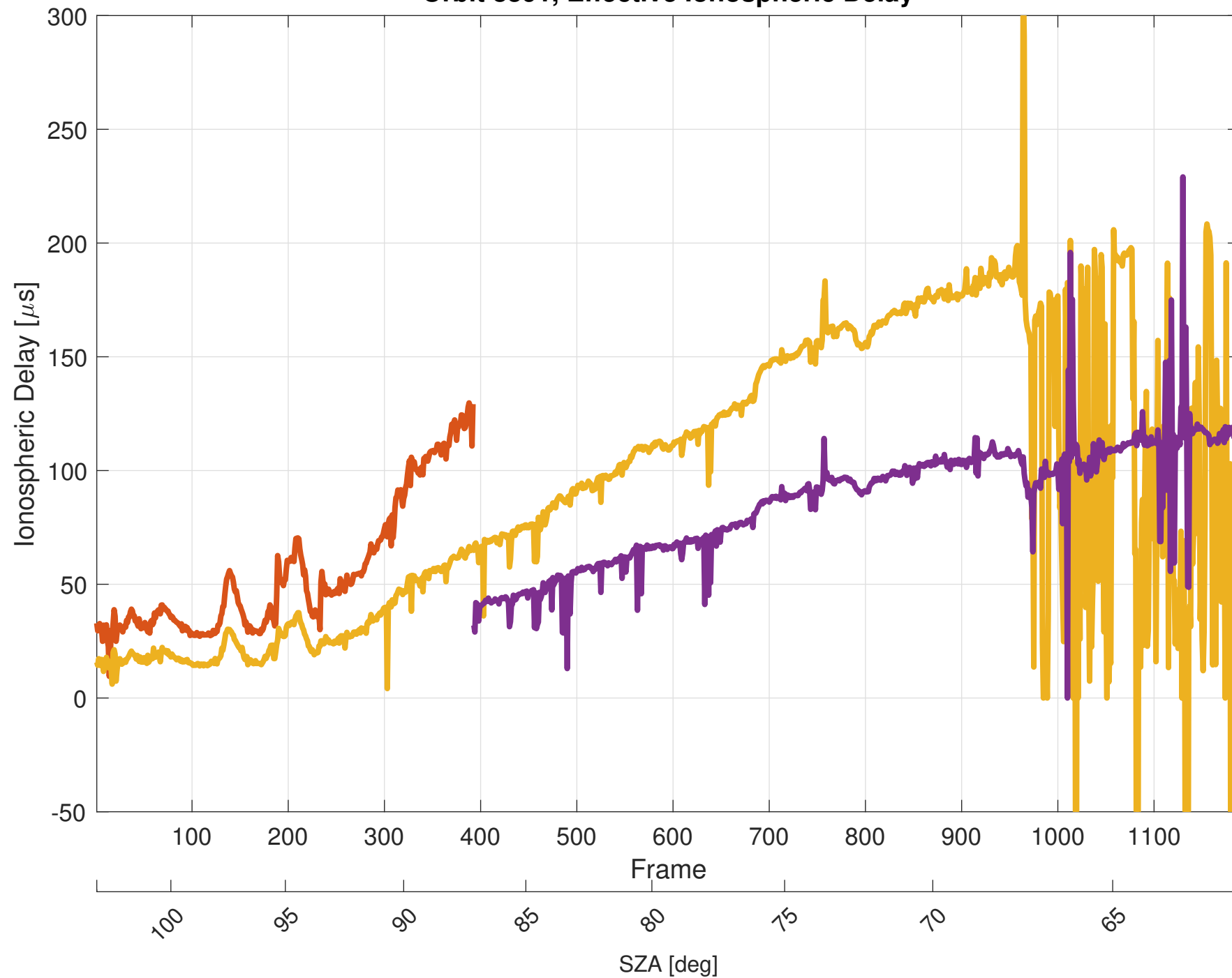
Orbit 8391, Effective Ionospheric Delay
