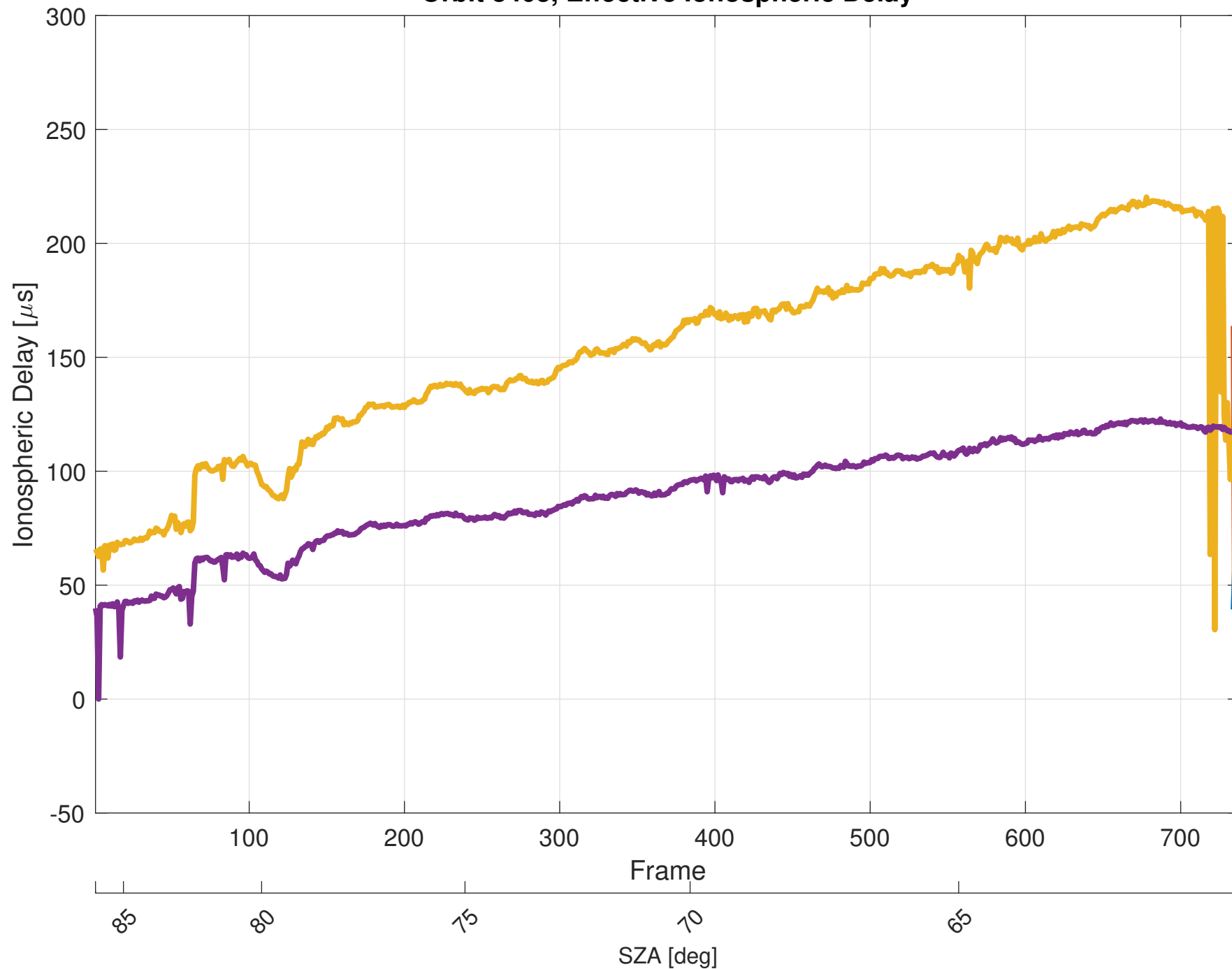
Orbit 8403, Effective Ionospheric Delay
