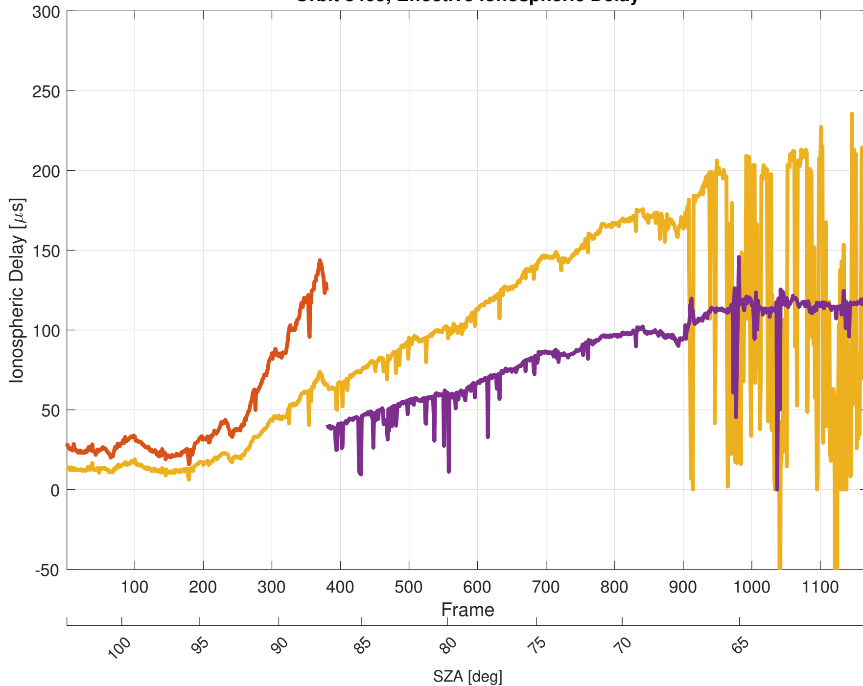
Orbit 8405, Effective Ionospheric Delay
