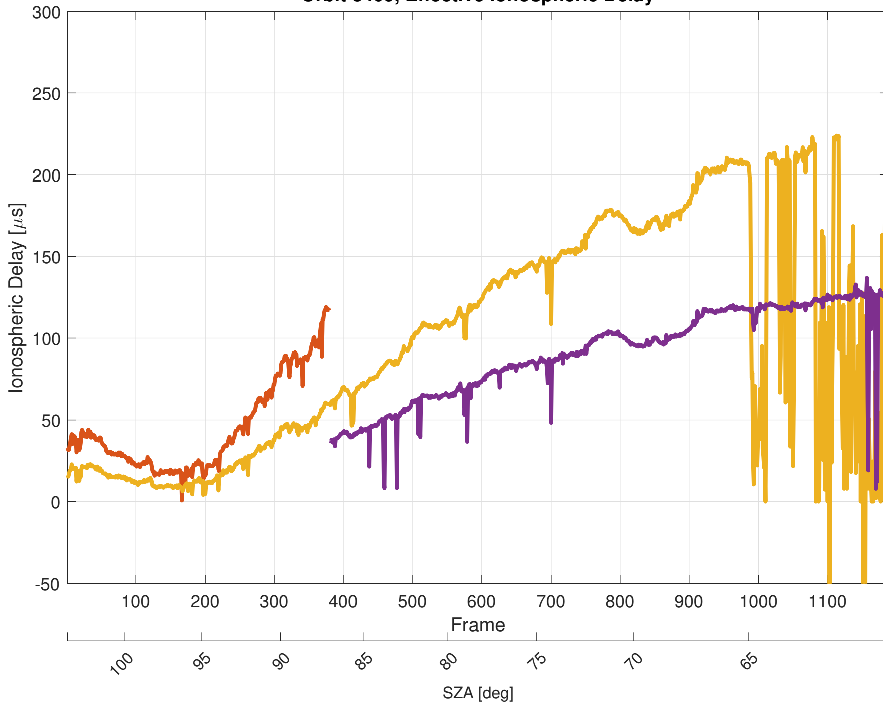
Orbit 8409, Effective Ionospheric Delay
