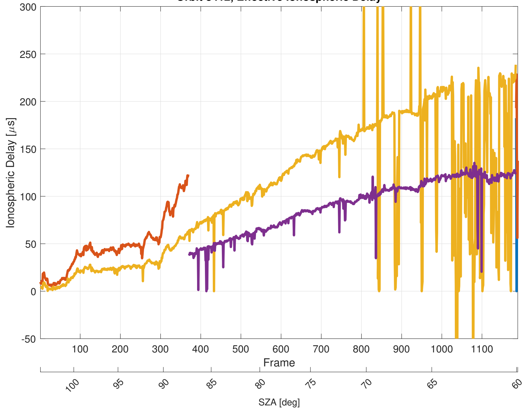
Orbit 8412, Effective Ionospheric Delay
