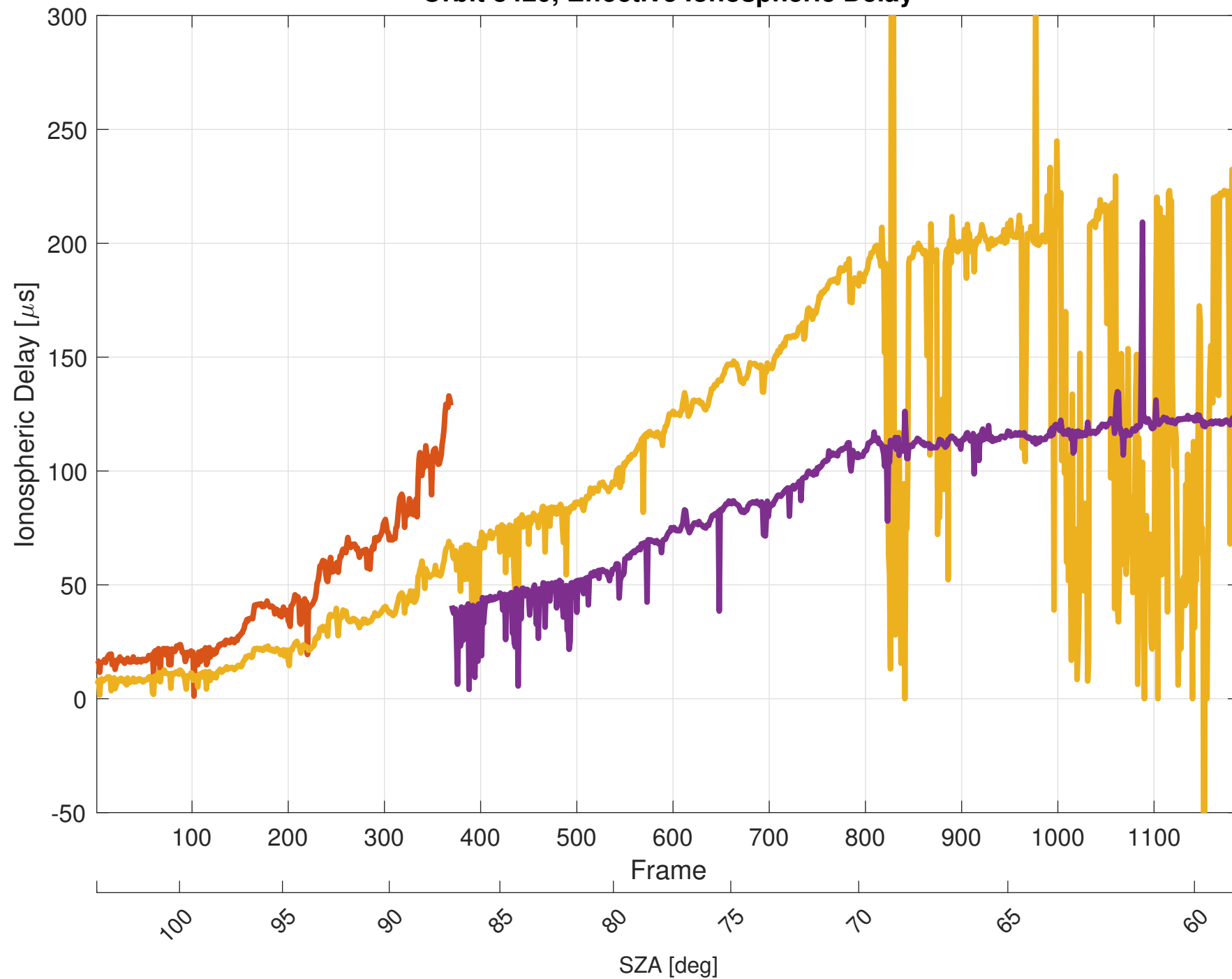
Orbit 8420, Effective Ionospheric Delay
