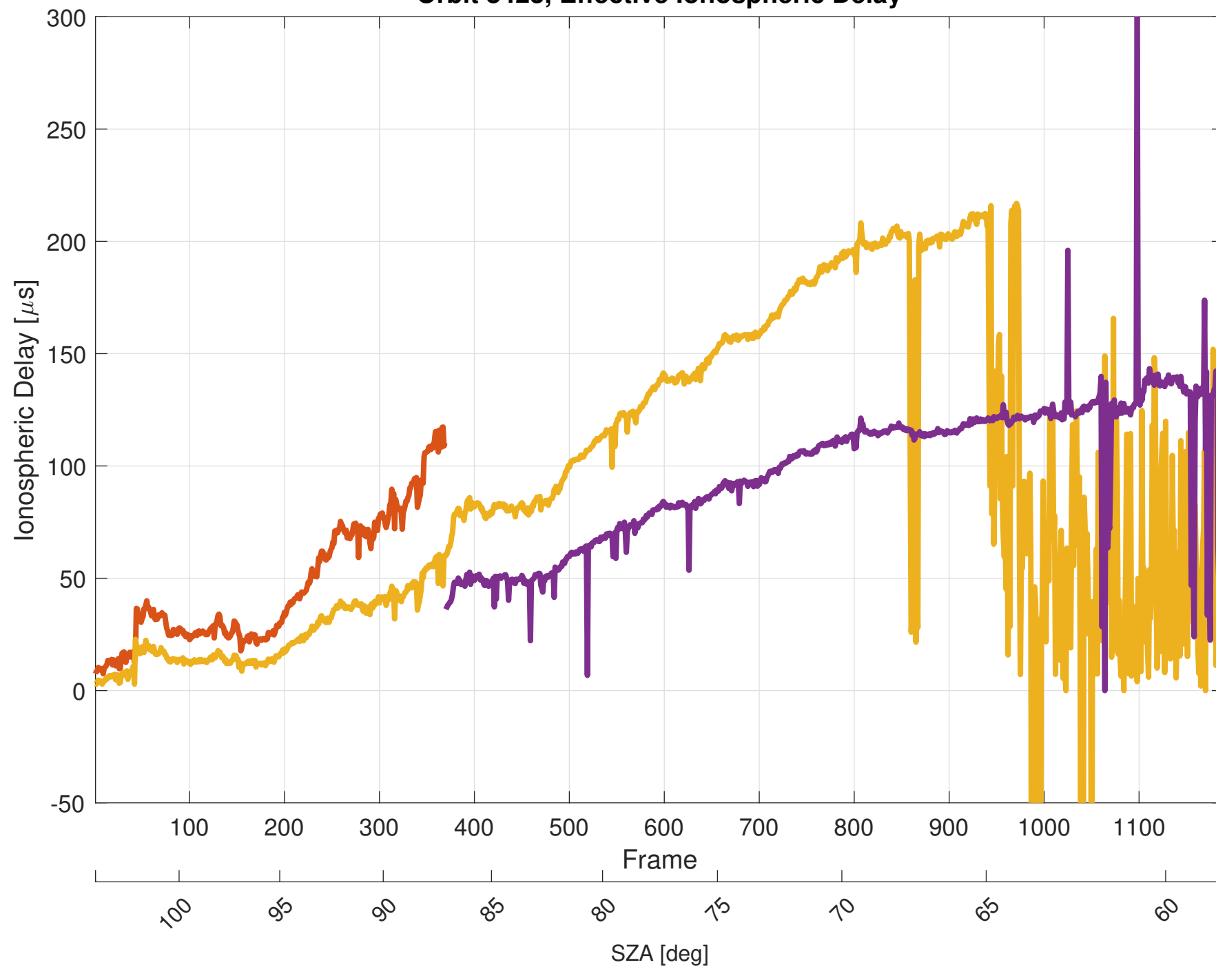
Orbit 8423, Effective Ionospheric Delay
