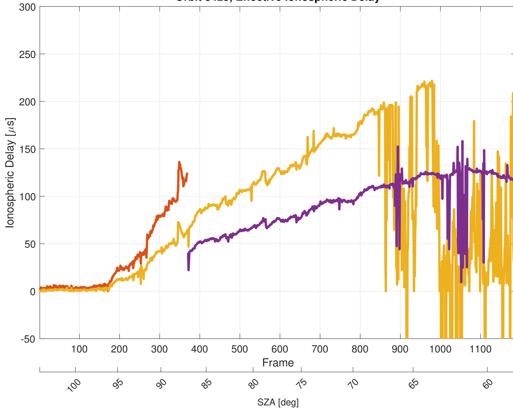
Orbit 8425, Effective Ionospheric Delay
