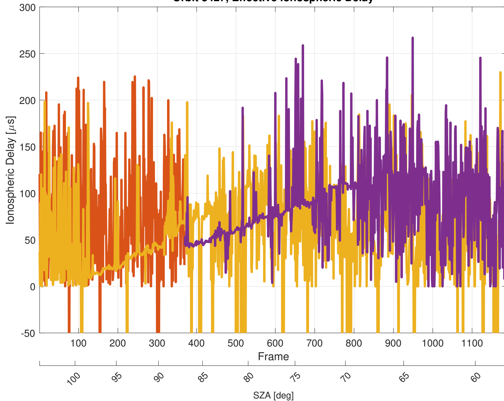
Orbit 8427, Effective Ionospheric Delay
