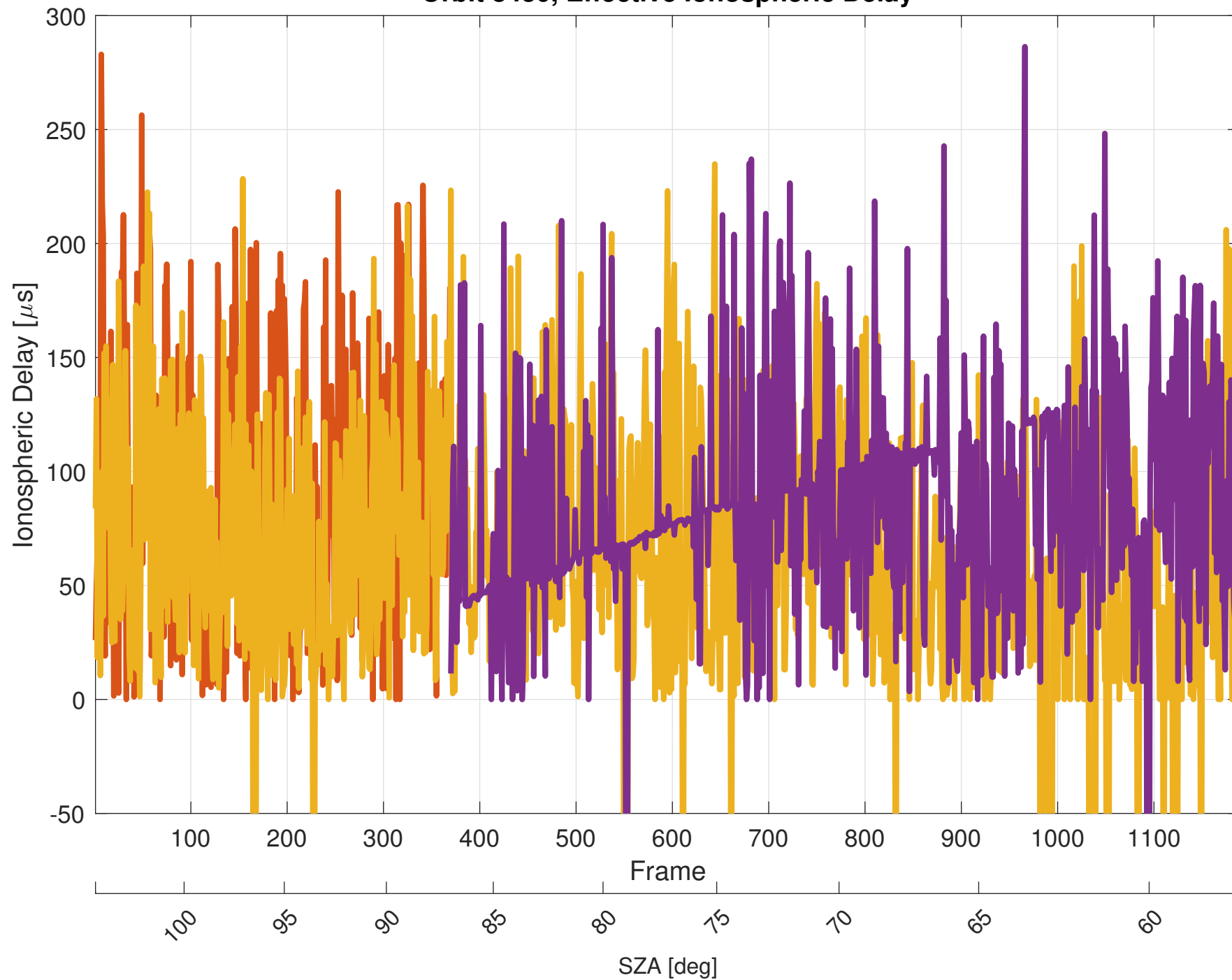
Orbit 8430, Effective Ionospheric Delay
