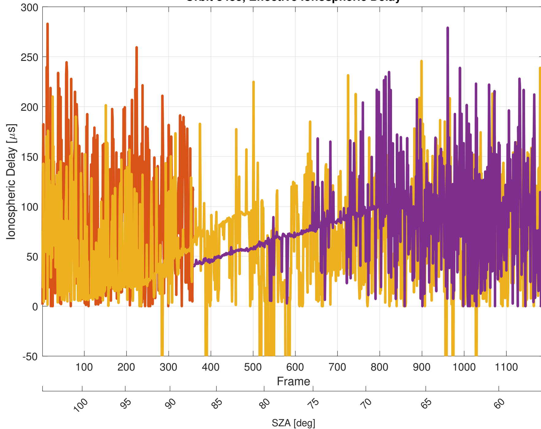
Orbit 8433, Effective Ionospheric Delay
