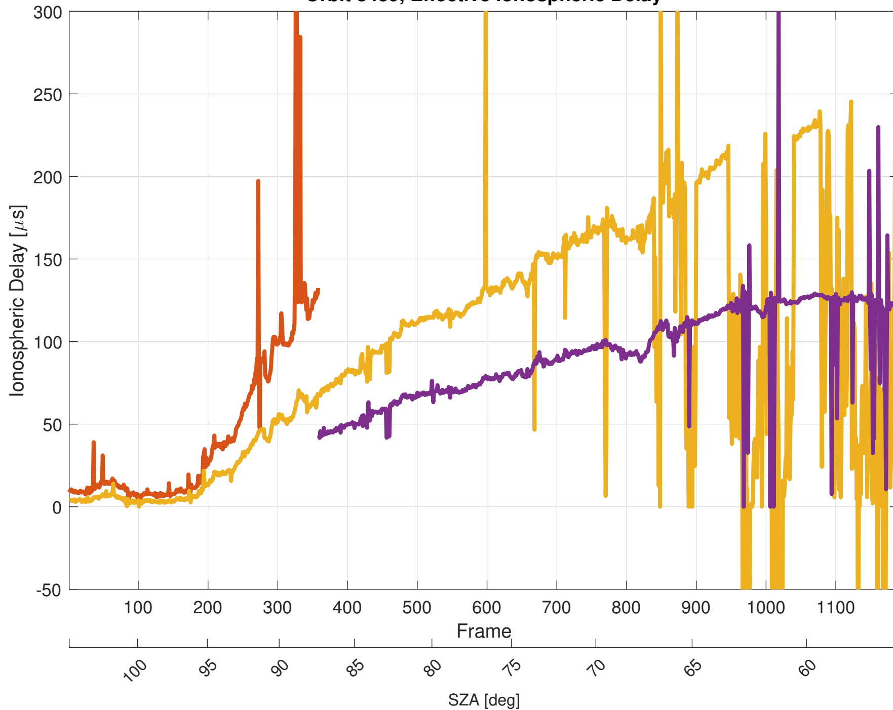
Orbit 8439, Effective Ionospheric Delay
