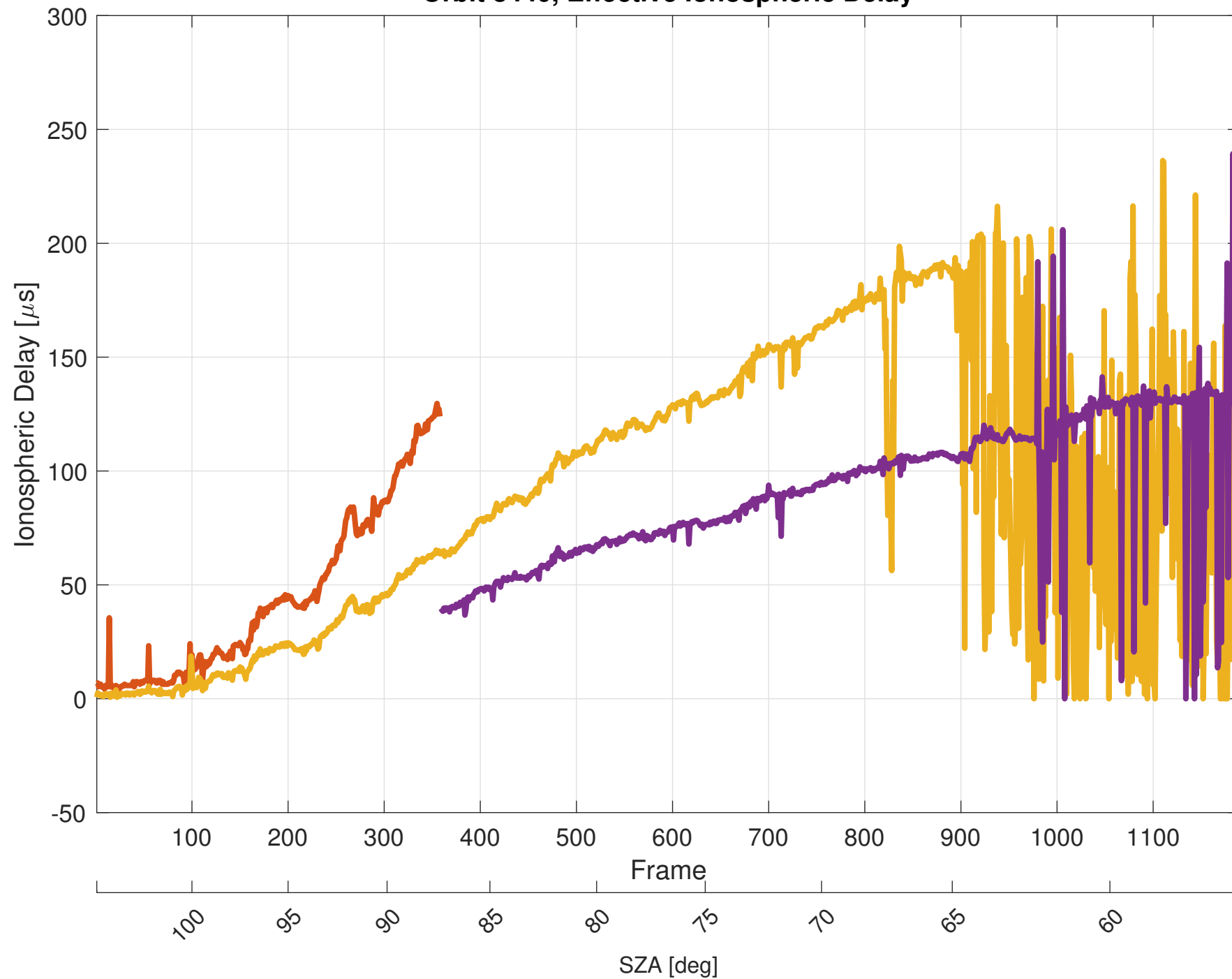
Orbit 8440, Effective Ionospheric Delay
