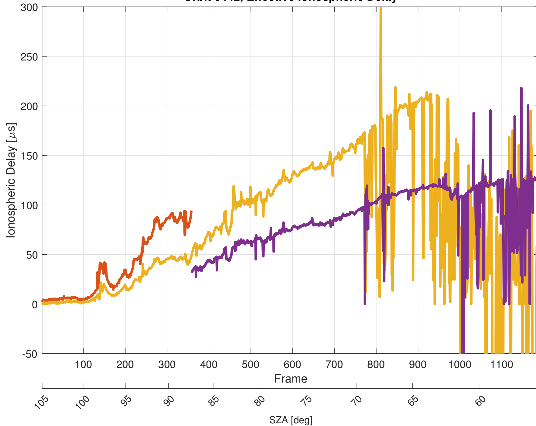
Orbit 8442, Effective Ionospheric Delay
