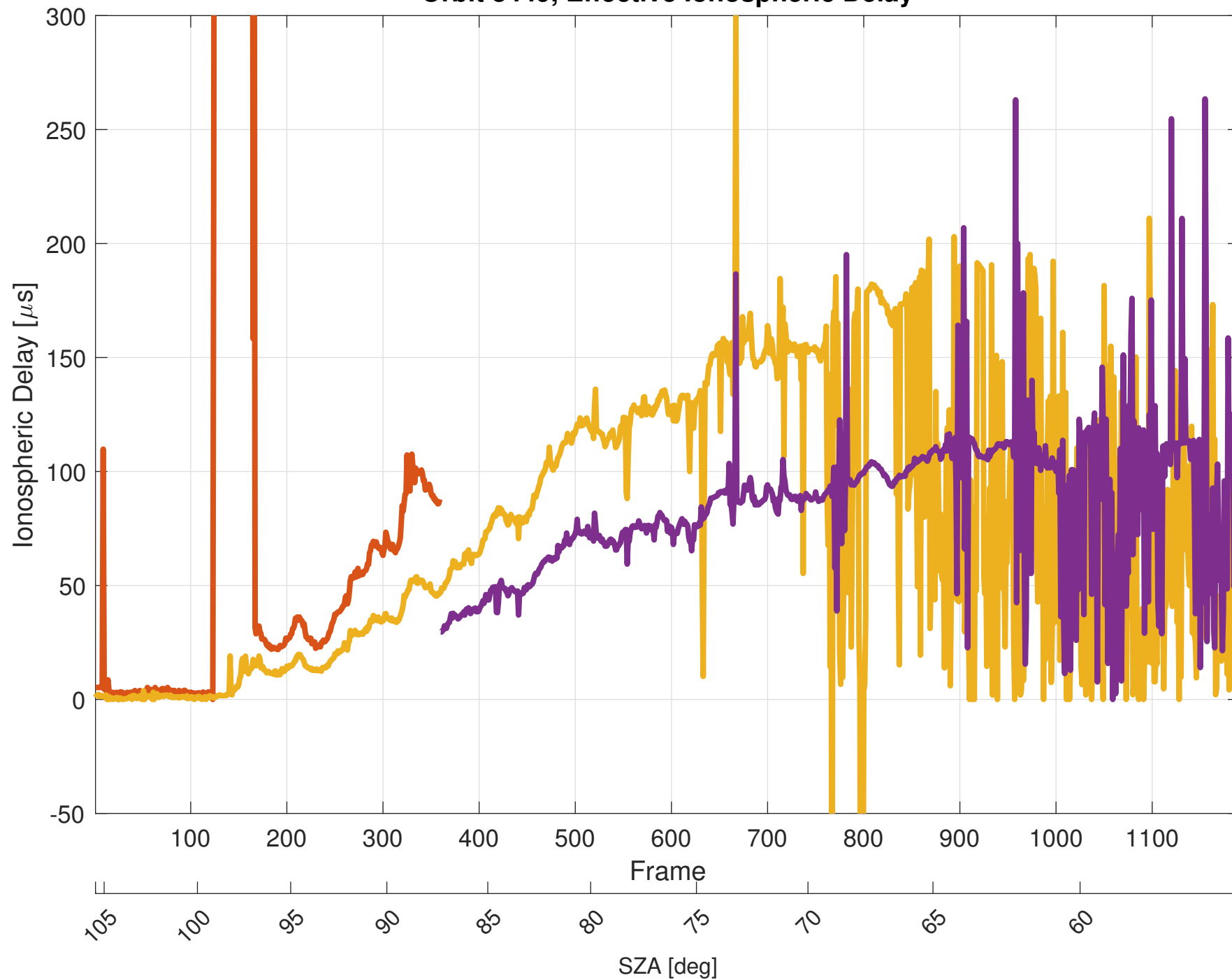
Orbit 8449, Effective Ionospheric Delay
