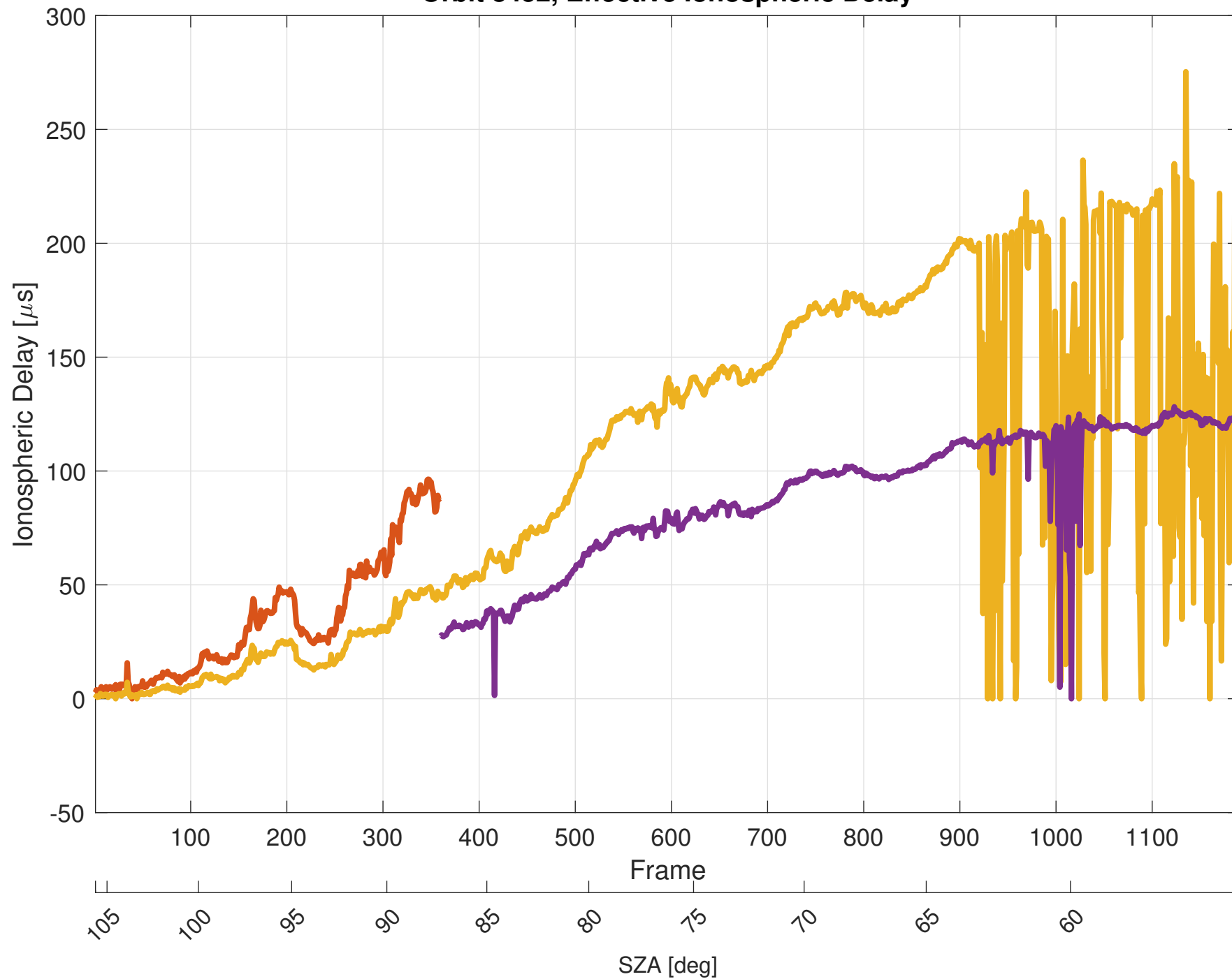
Orbit 8452, Effective Ionospheric Delay
