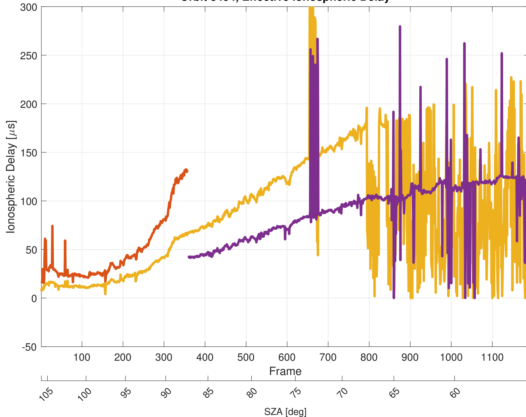
Orbit 8454, Effective Ionospheric Delay
