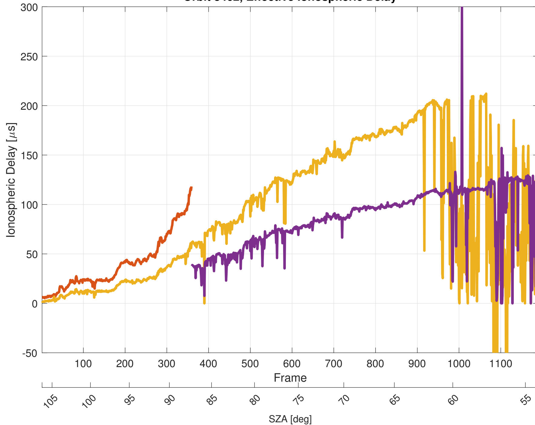
Orbit 8462, Effective Ionospheric Delay
