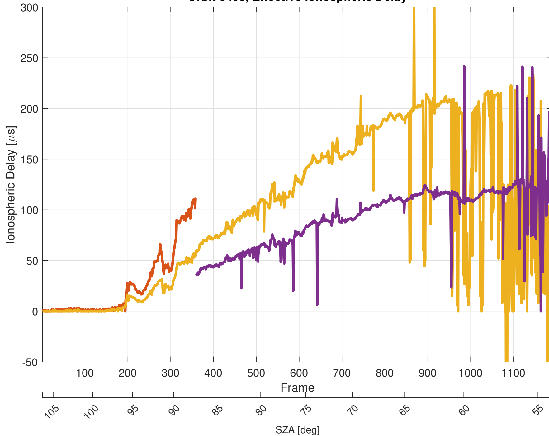
Orbit 8463, Effective Ionospheric Delay
