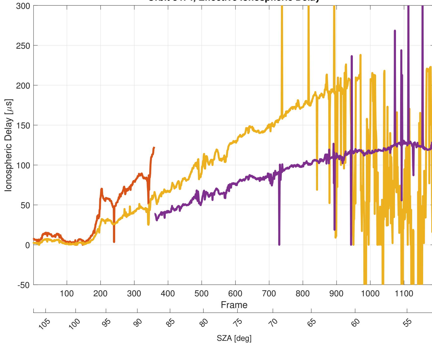
Orbit 8474, Effective Ionospheric Delay
