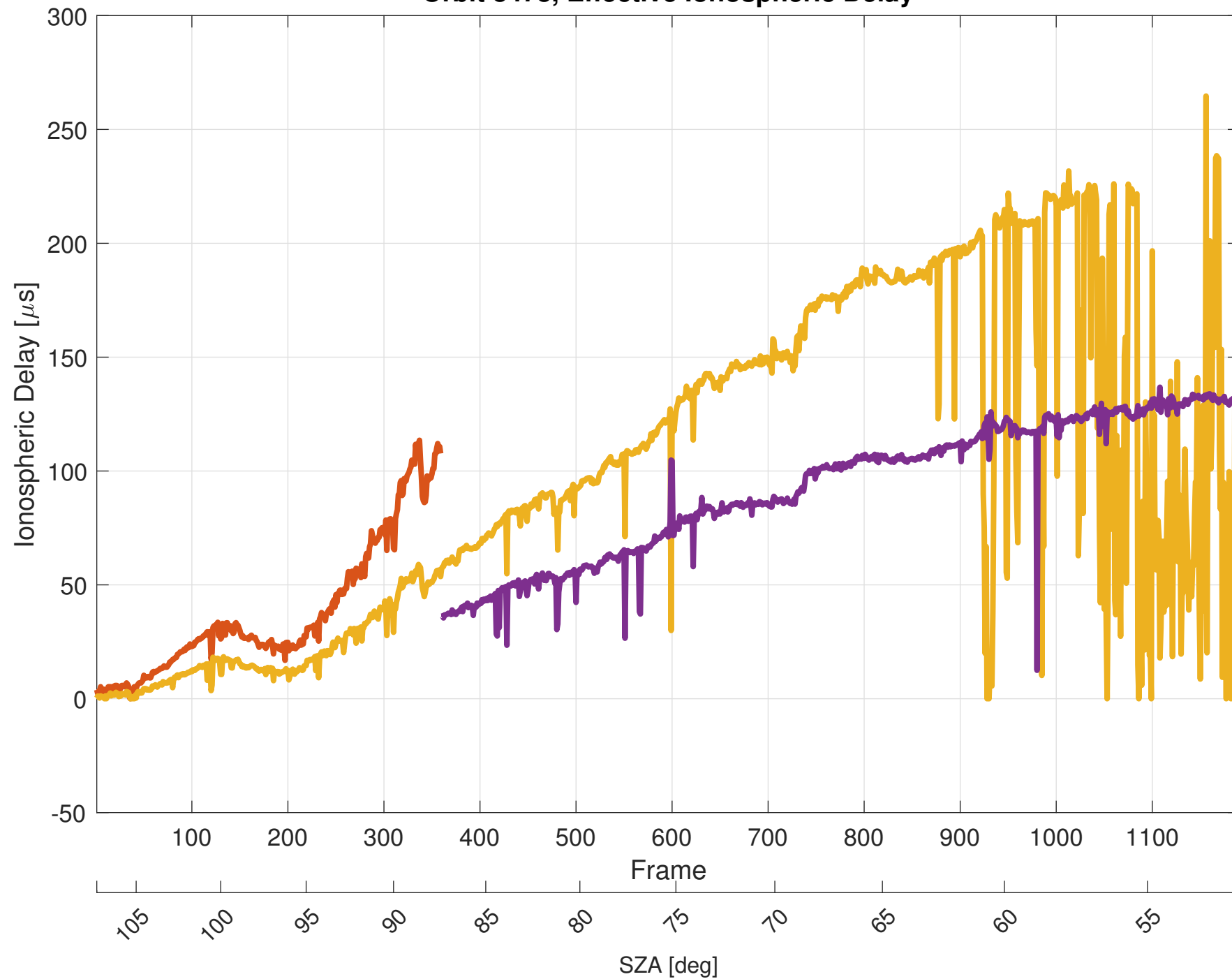
Orbit 8478, Effective Ionospheric Delay
