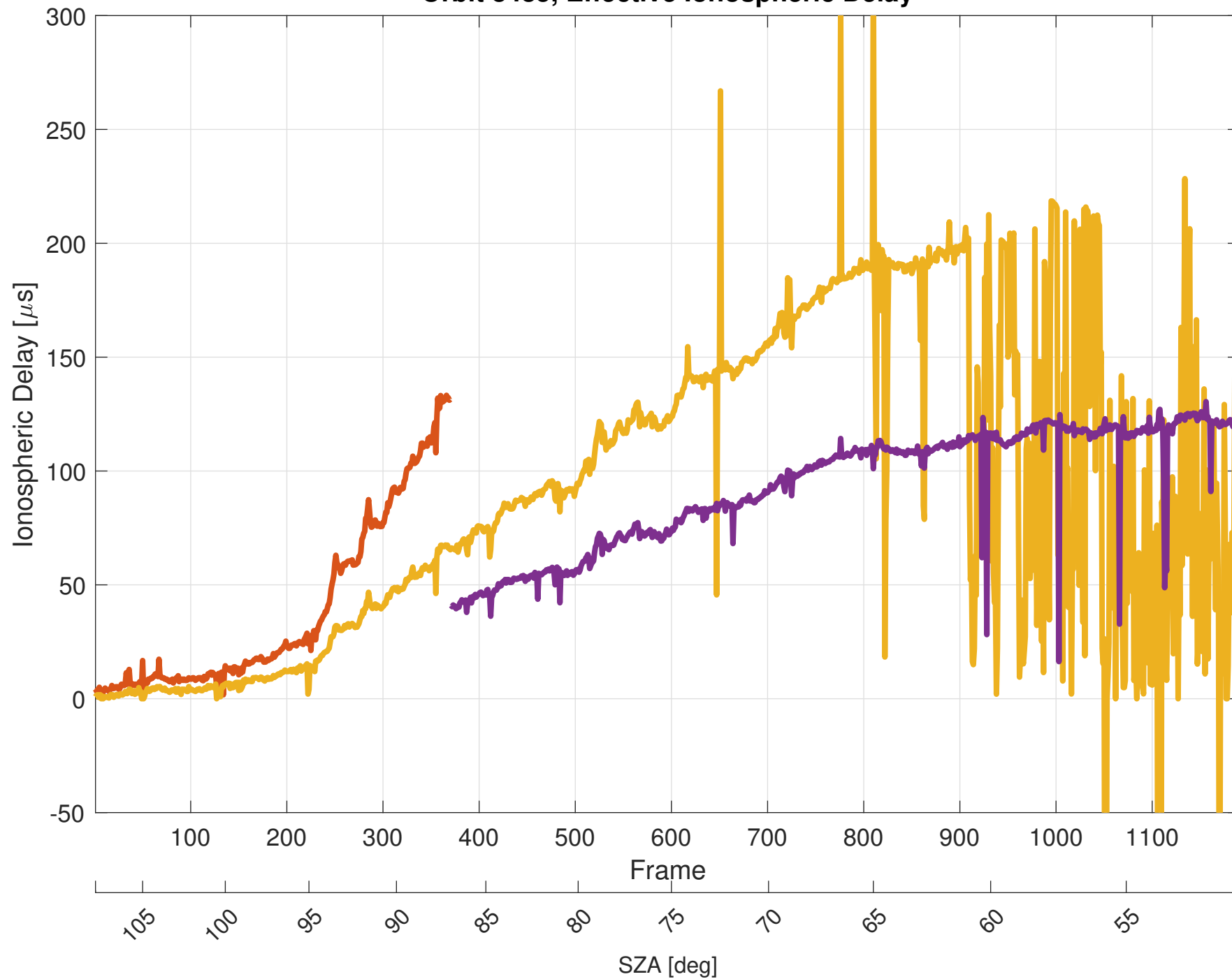
Orbit 8485, Effective Ionospheric Delay
