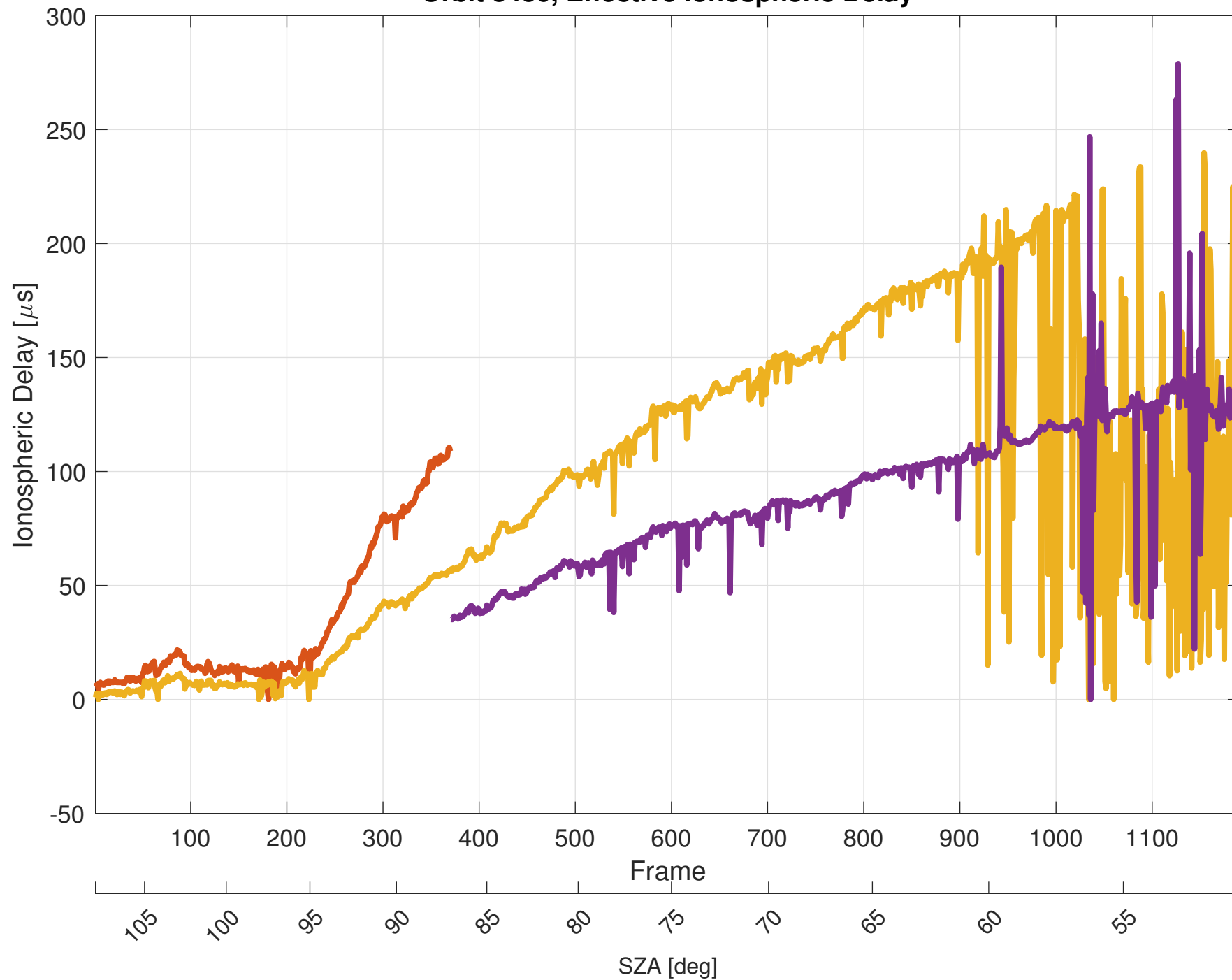
Orbit 8486, Effective Ionospheric Delay
