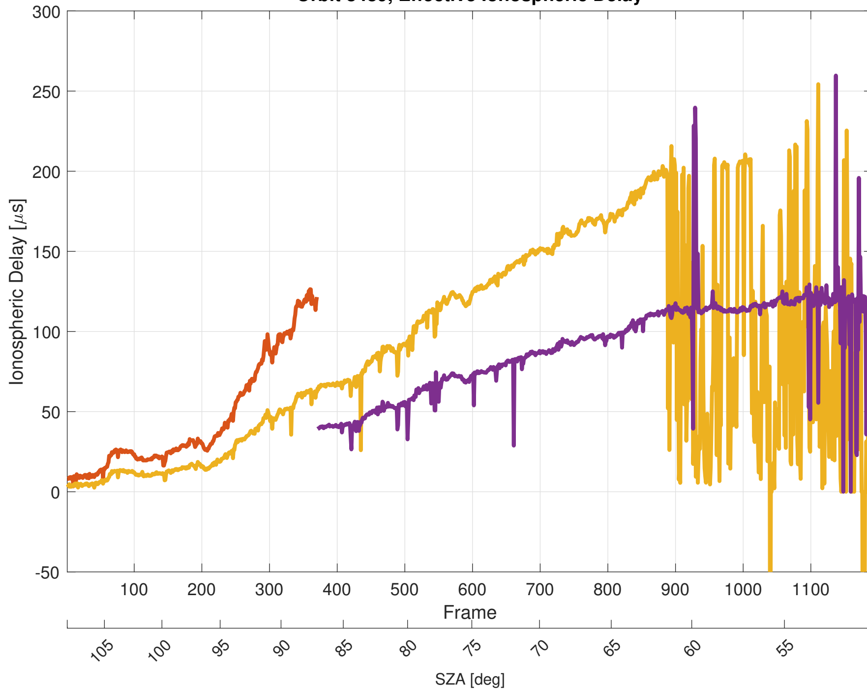
Orbit 8489, Effective Ionospheric Delay
