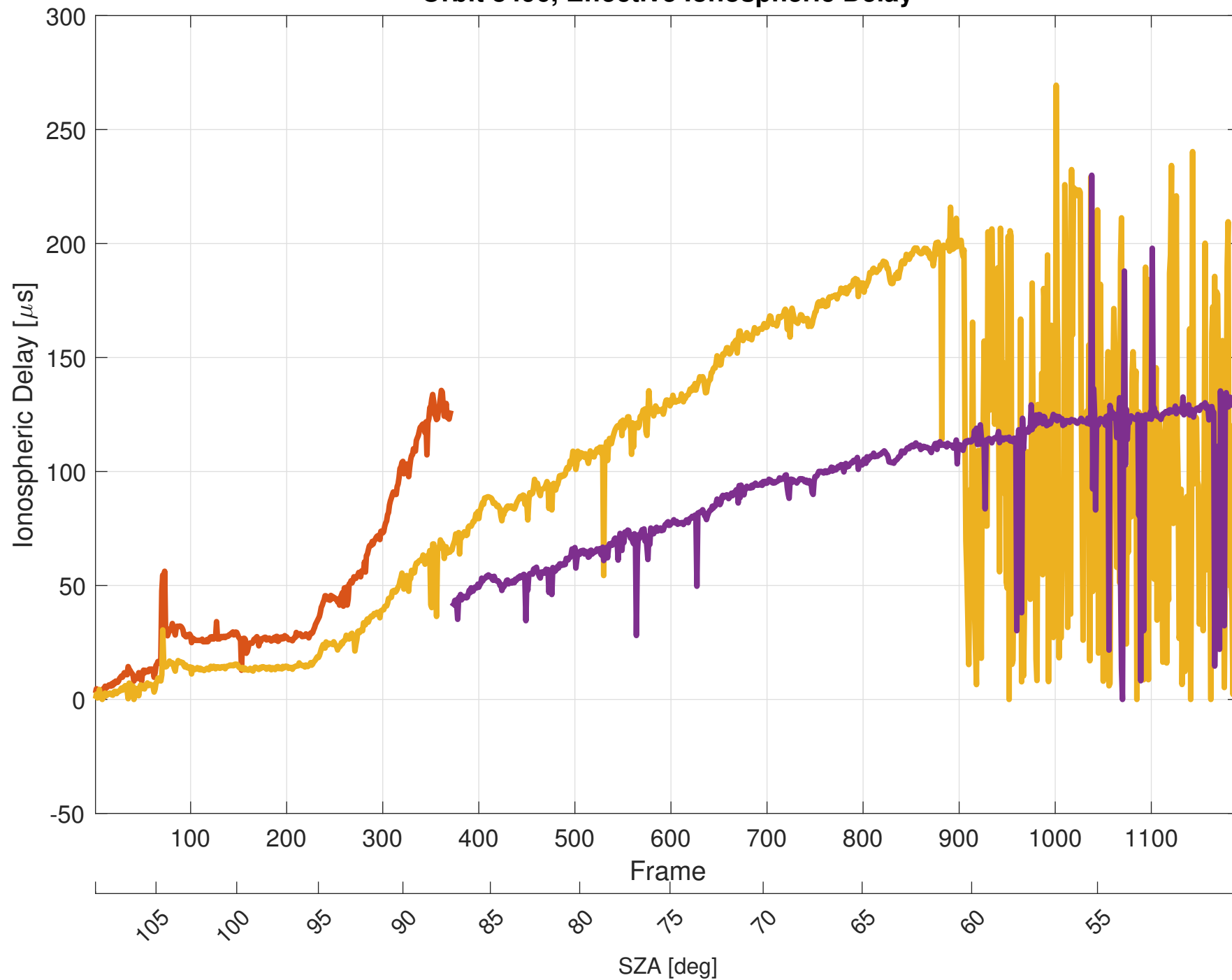
Orbit 8496, Effective Ionospheric Delay
