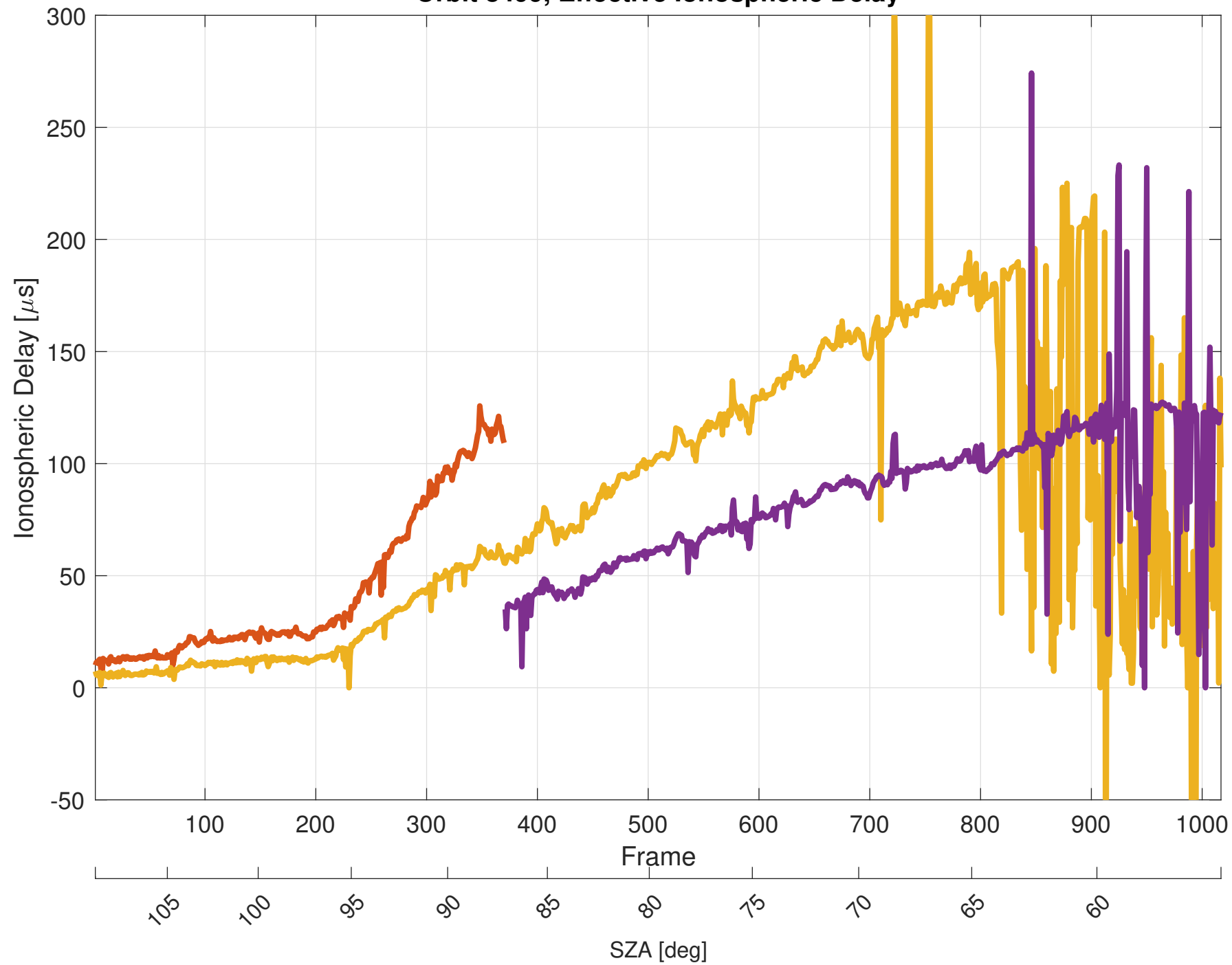
Orbit 8499, Effective Ionospheric Delay
