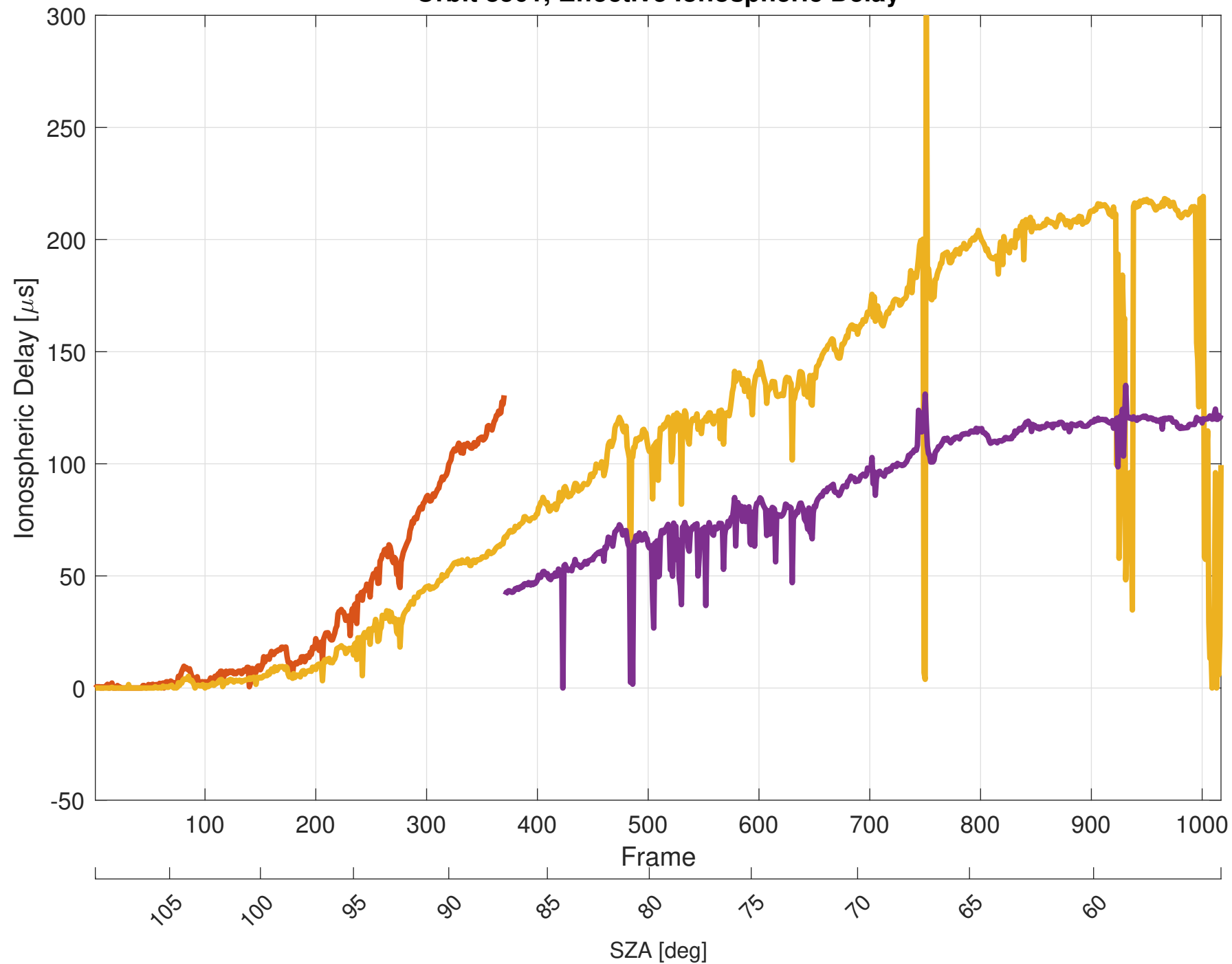
Orbit 8501, Effective Ionospheric Delay
