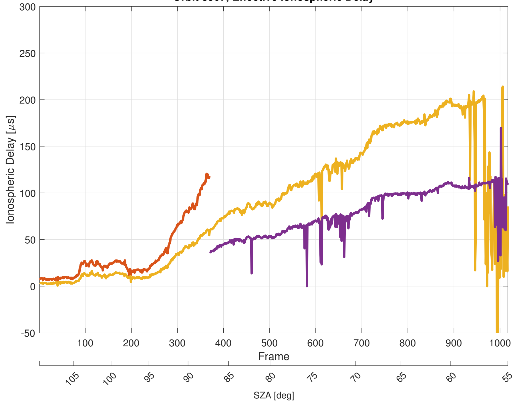
Orbit 8507, Effective Ionospheric Delay
