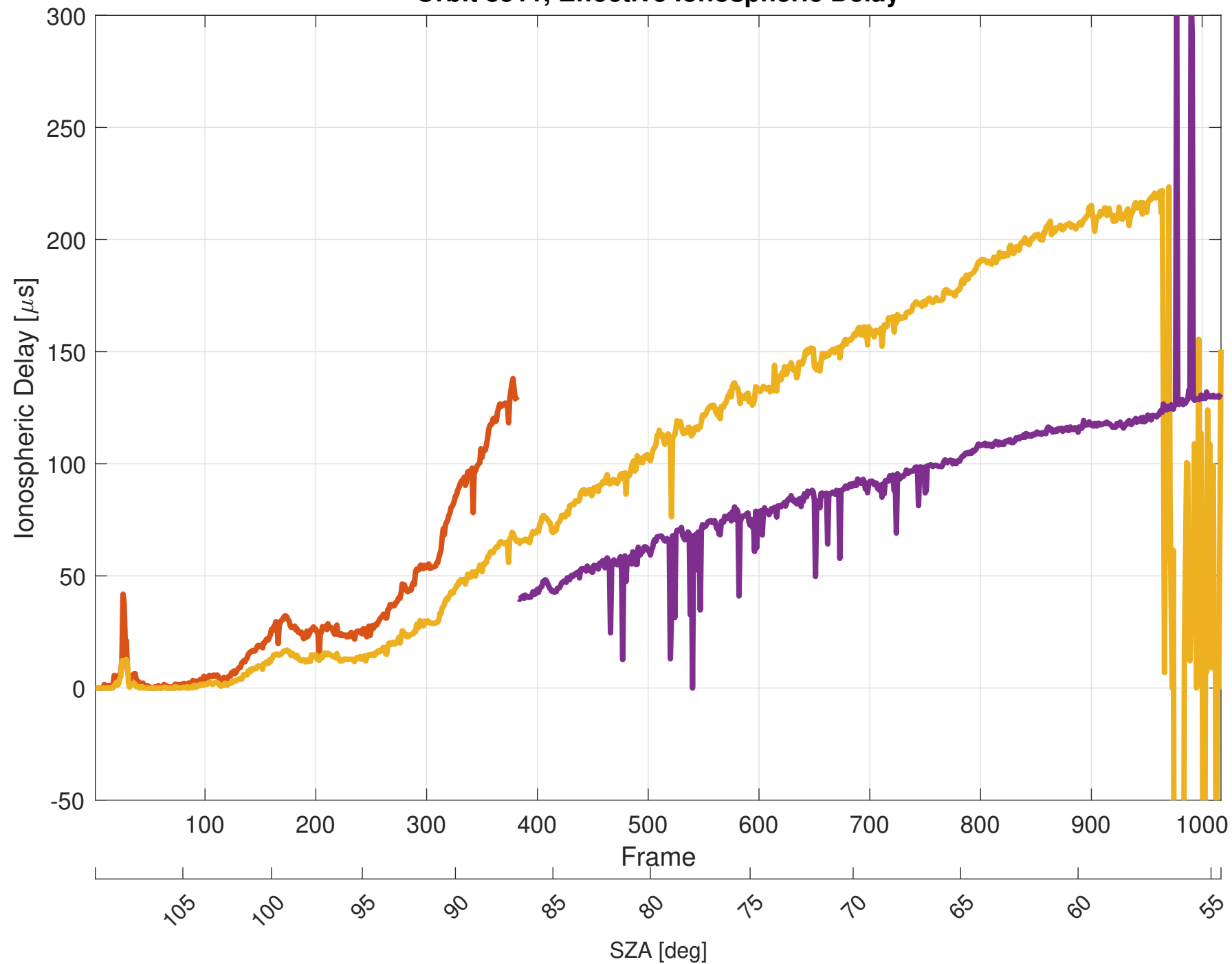
Orbit 8511, Effective Ionospheric Delay
