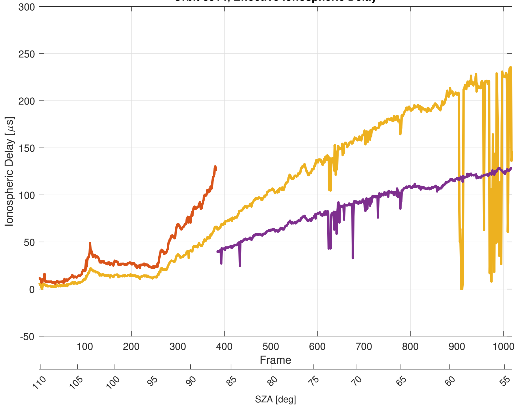
Orbit 8514, Effective Ionospheric Delay
