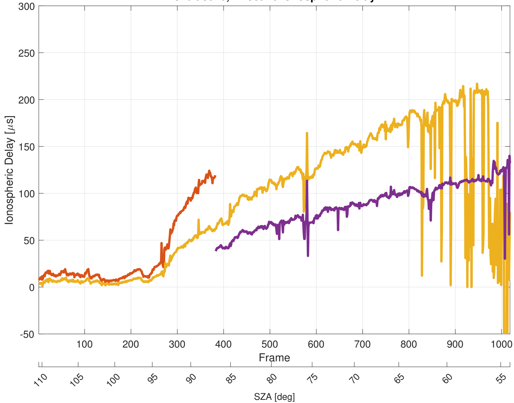
Orbit 8516, Effective Ionospheric Delay
