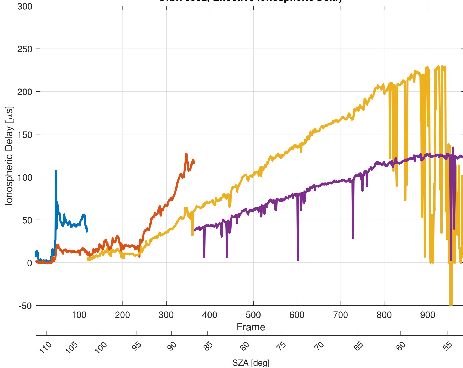
Orbit 8532, Effective Ionospheric Delay
