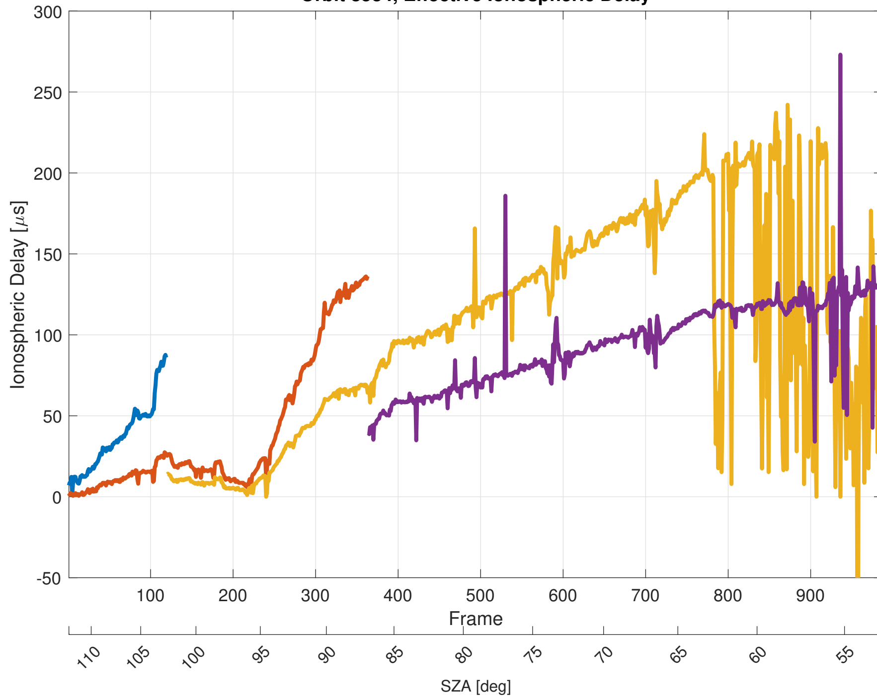
Orbit 8534, Effective Ionospheric Delay
