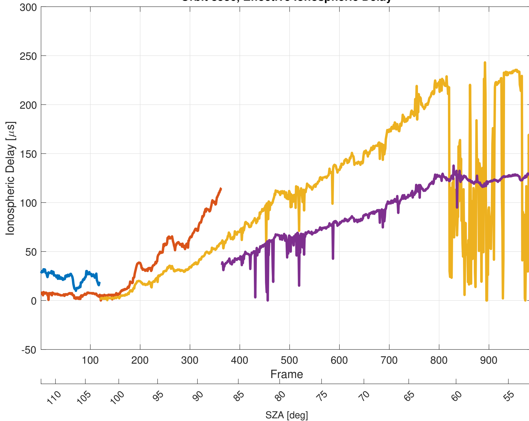
Orbit 8536, Effective Ionospheric Delay
