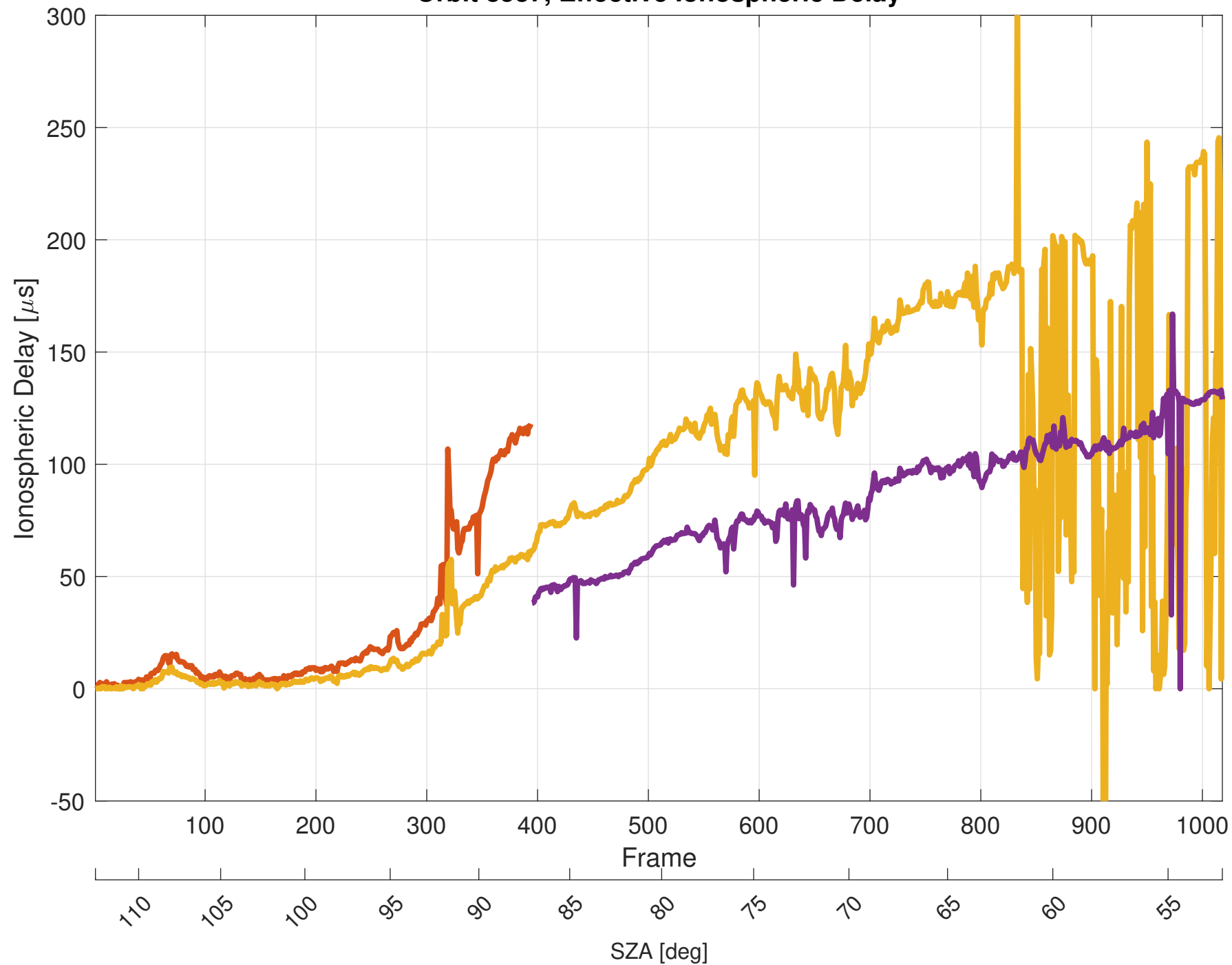
Orbit 8537, Effective Ionospheric Delay
